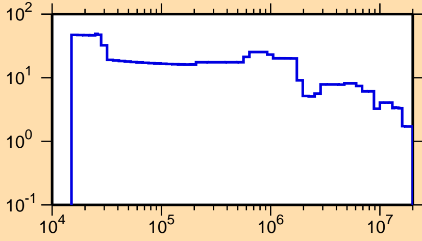
\Delta\sigma/\sigma vs. E for ^{198}\text{At}(n, tot.)
