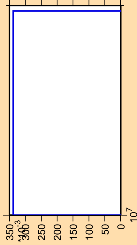
\Delta\sigma/\sigma vs. E for ^{198}\text{At}(n,3n\alpha)
