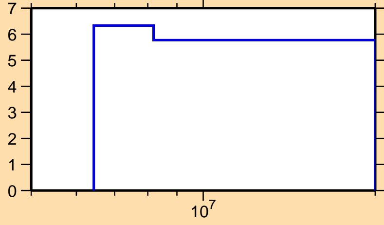
\Delta\sigma/\sigma vs. E for ^{198}\text{At}(n,\text{nonel.})
