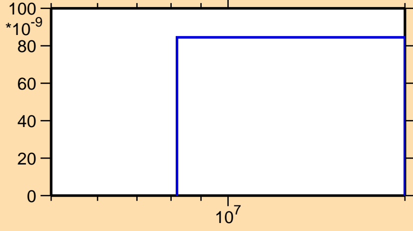
\sigma vs. E for ^{198}\text{At}(n,\text{pd})
