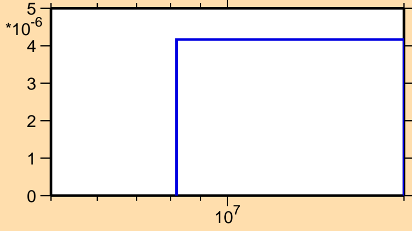
\sigma vs. E for ^{198}\text{At}(n,2np)
