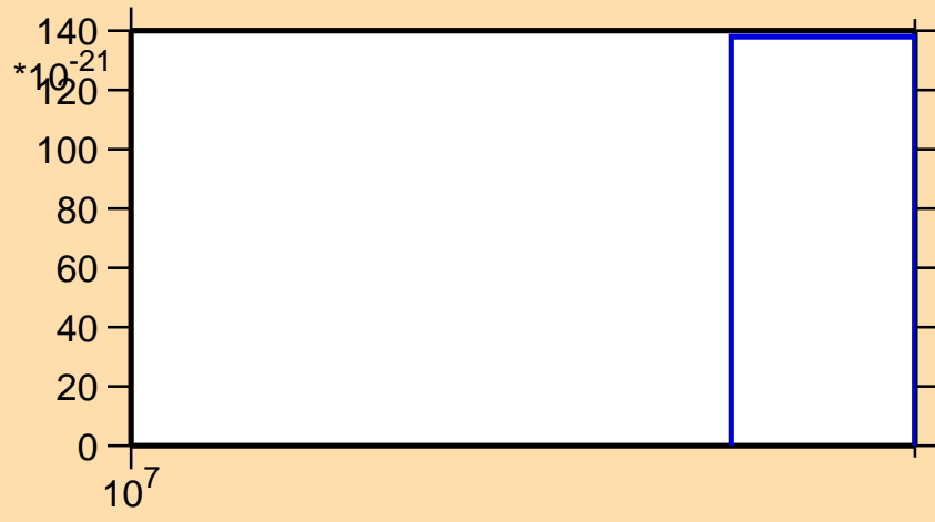
\sigma vs. E for ^{199}\text{At}(\text{mt } 42)
