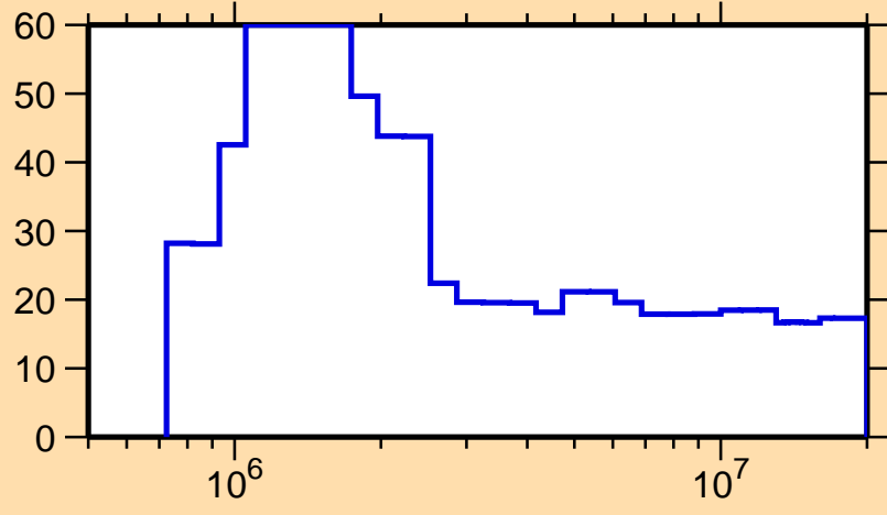
\Delta\sigma/\sigma vs. E for ^{199}\text{At}(n,n\text{cont.})
