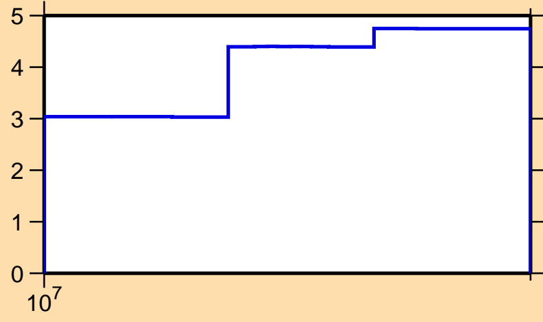
\Delta\sigma/\sigma vs. E for ^{199}\text{At}(n,\text{el.})
