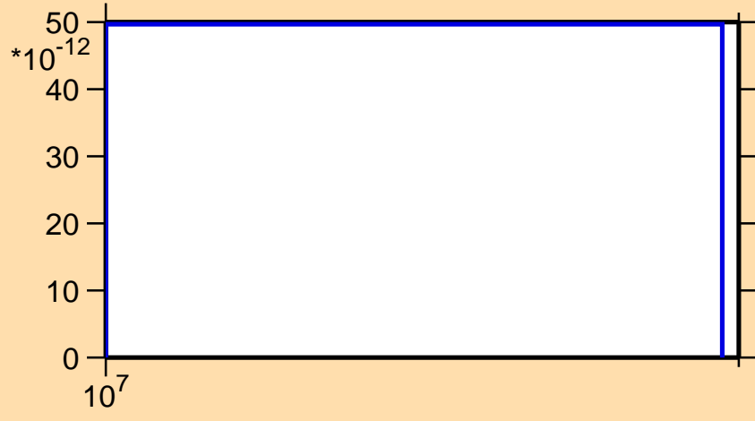
\sigma vs. E for ^{199}\text{At}(n,\text{pt})
