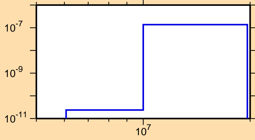
\sigma vs. E for ^{199}\text{At}(\text{mt } 45)
