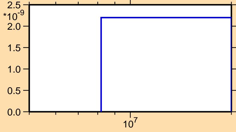
\sigma vs. E for ^{199}\text{At}(\text{mt117})
