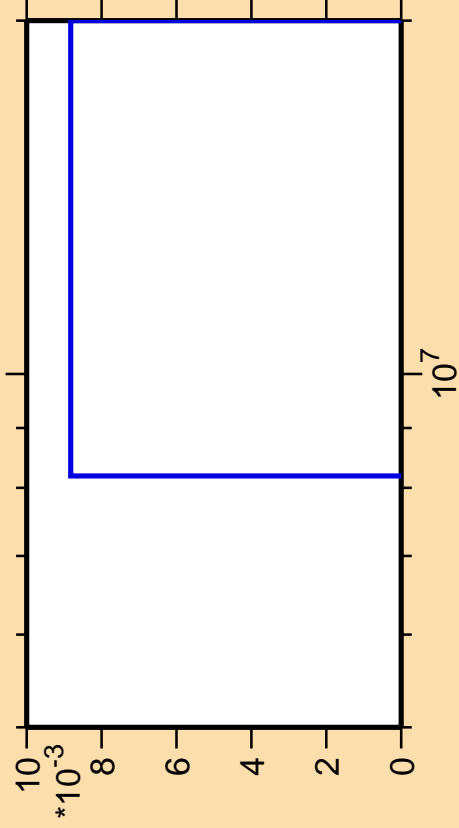
\Delta\sigma/\sigma vs. E for ^{199}\text{At}(n,3n\alpha)
