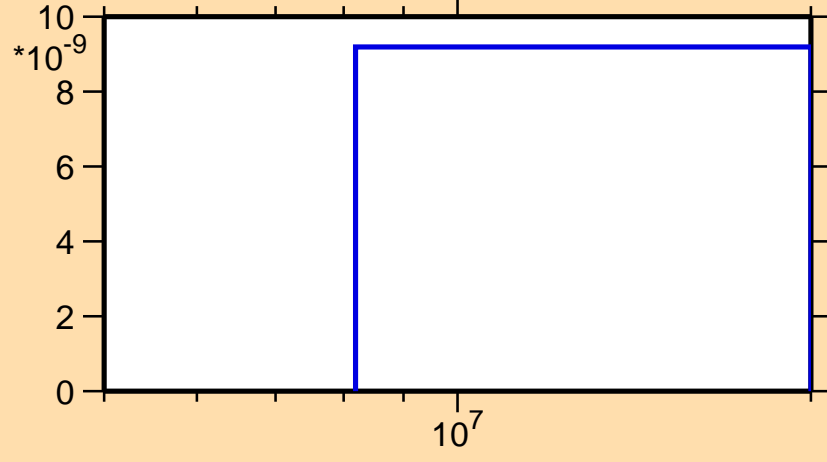
\sigma vs. E for ^{199}\text{At}(n,\text{nd})
