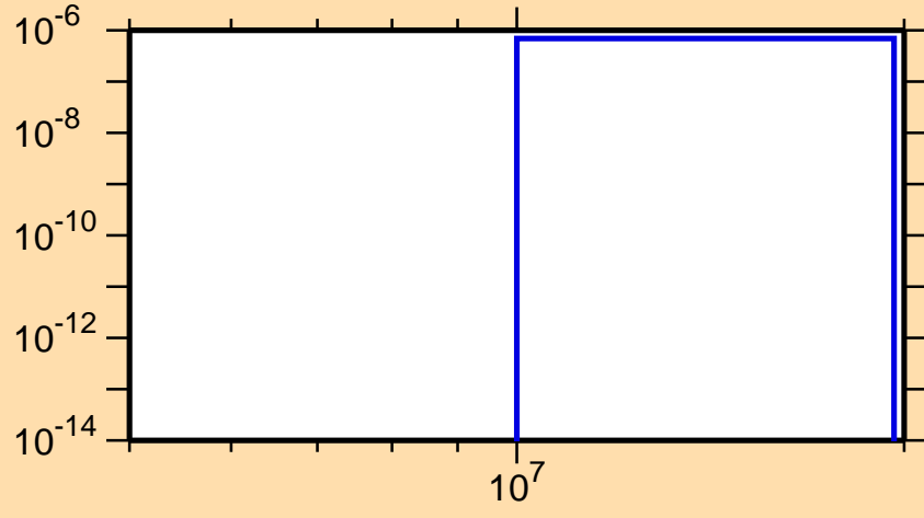
\sigma vs. E for ^{200}\text{At}(n,nd)
