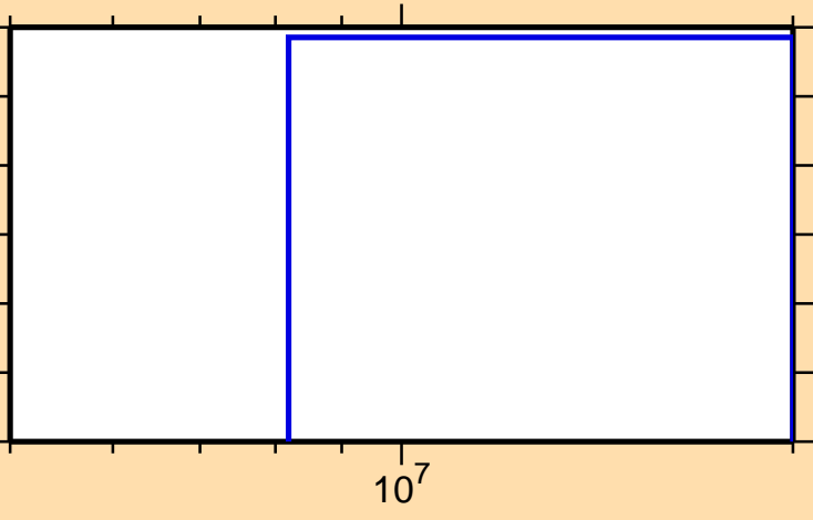
\sigma vs. E for ^{200}\text{At}(n,\text{pd})
