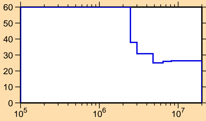
\Delta\sigma/\sigma vs. E for ^{200}\text{At}(n,ncont.)
