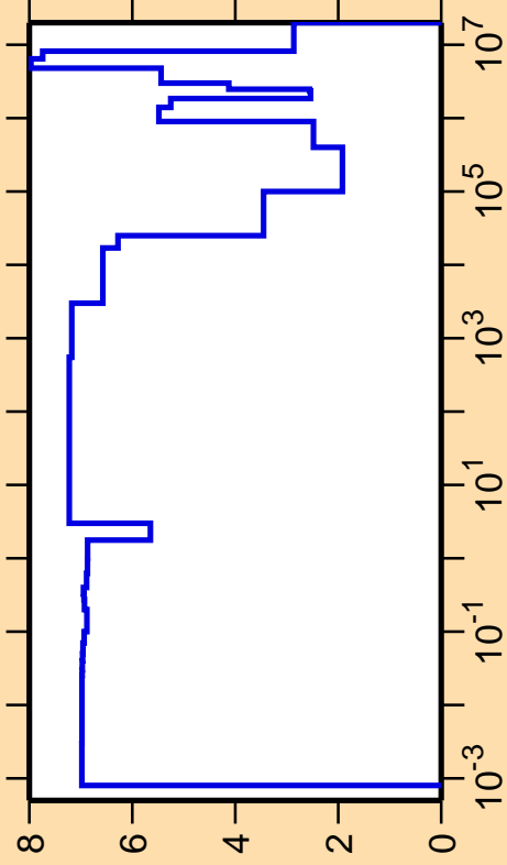
\Delta\sigma/\sigma vs. E for ^{200}\text{At}(n,\text{el.})
