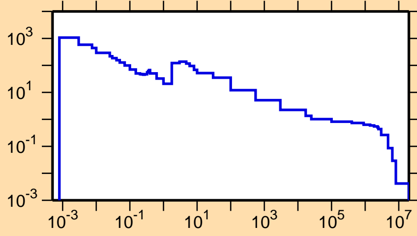
\sigma vs. E for ^{200}\text{At}(n,\gamma)
