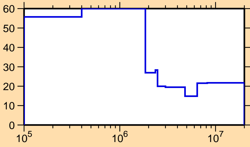
\Delta\sigma/\sigma vs. E for ^{200}\text{At}(n,n_1)
