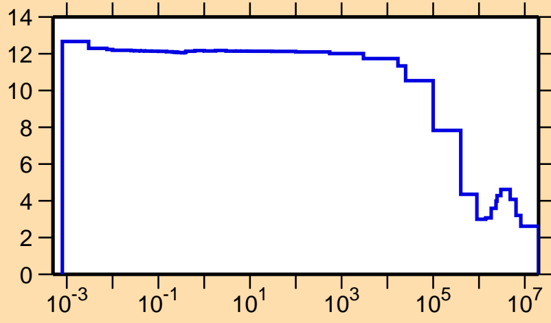
\sigma vs. E for ^{200}\text{At}(n,\text{el.})
