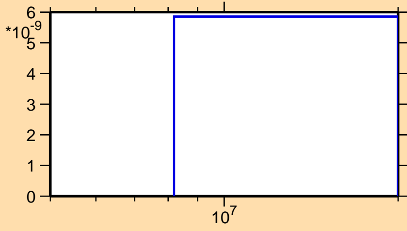
\sigma vs. E for ^{200}\text{At}(n,\text{pd})
