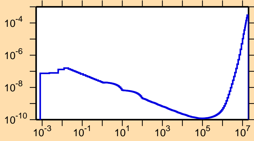
\sigma vs. E for ^{200}\text{At}(n,p\alpha)
