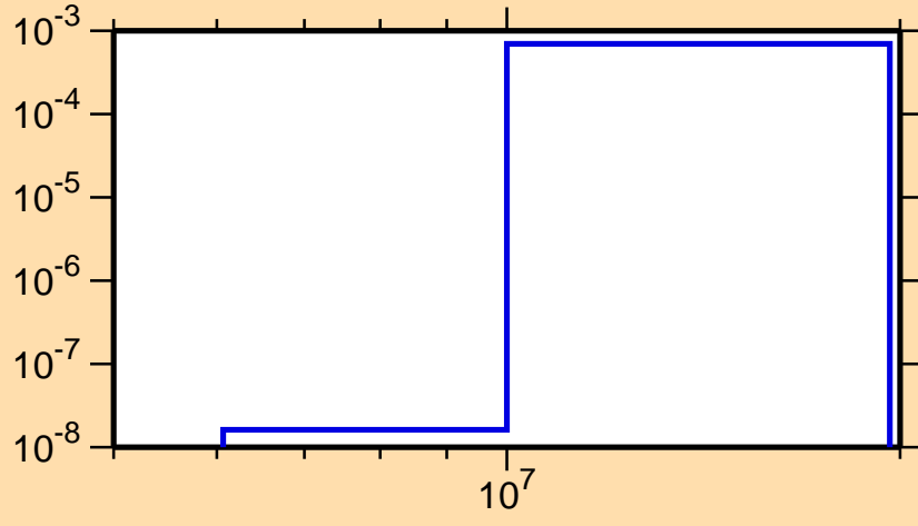
\sigma vs. E for ^{200}\text{At}(n,t)
