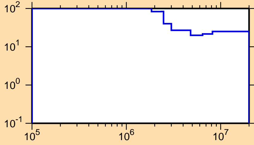
\Delta\sigma/\sigma vs. E for ^{200}\text{At}(n,ncont.)
