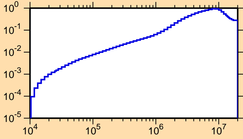
\sigma vs. E for ^{200}\text{At}(n,n\text{cont.})
