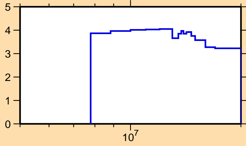
\Delta\sigma/\sigma vs. E for ^{200}\text{At}(n,\text{nonel.})
