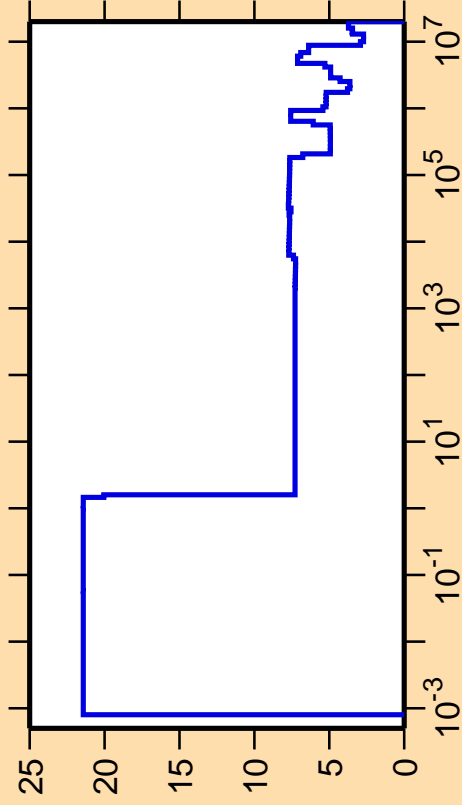
\Delta\sigma/\sigma vs. E for ^{200}\text{At}(n,\text{el.})
