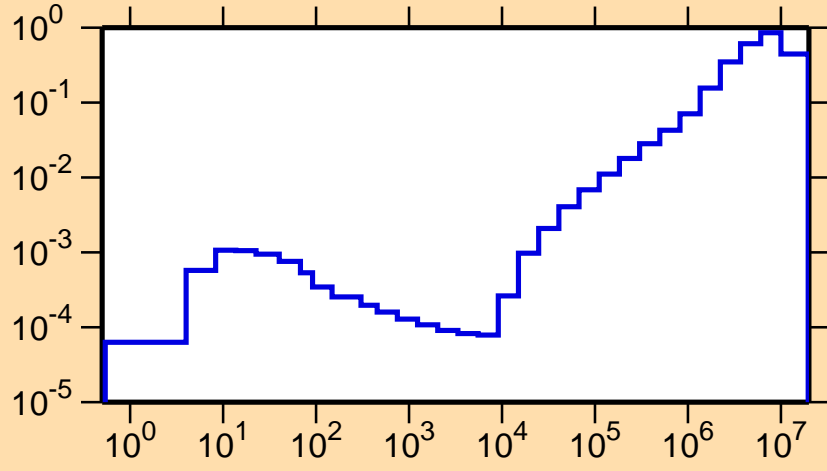
\sigma vs. E for ^{200}\text{At}(n,\text{inel.})
