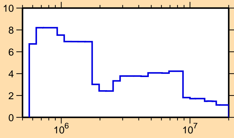
\Delta\sigma/\sigma vs. E for ^{201}\text{At}(n,\text{tot.})
