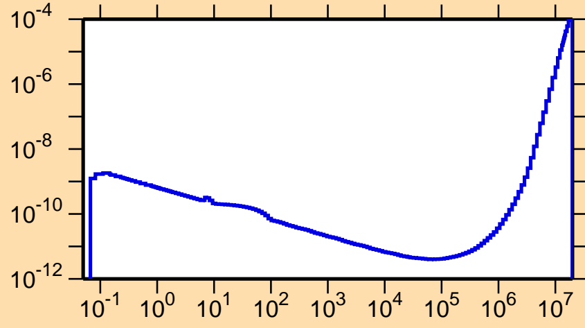
\sigma vs. E for ^{201}\text{At}(n,p\alpha)
