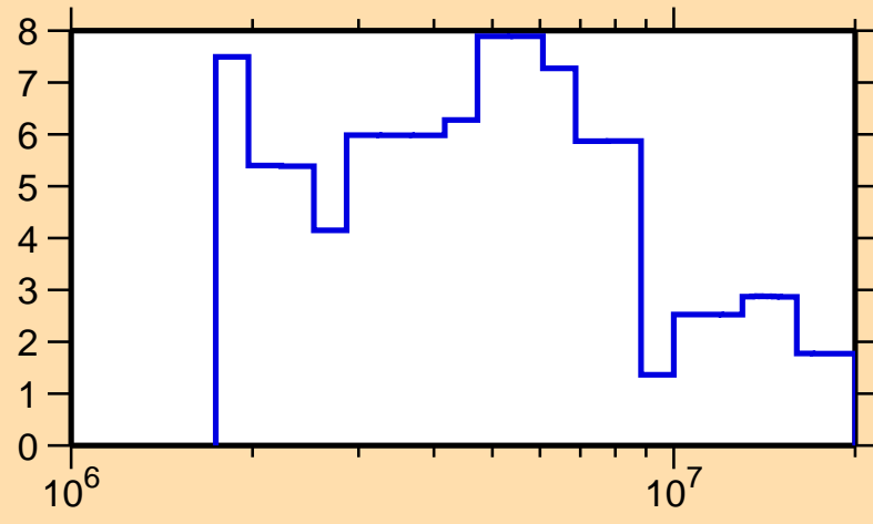
\Delta\sigma/\sigma vs. E for ^{201}\text{At}(n, el.)
