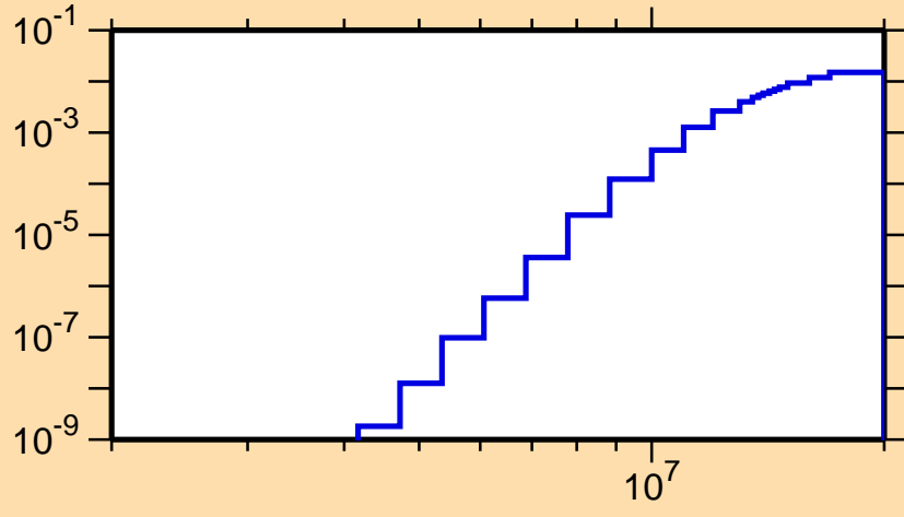
\sigma vs. E for ^{201}\text{At}(n,d)
