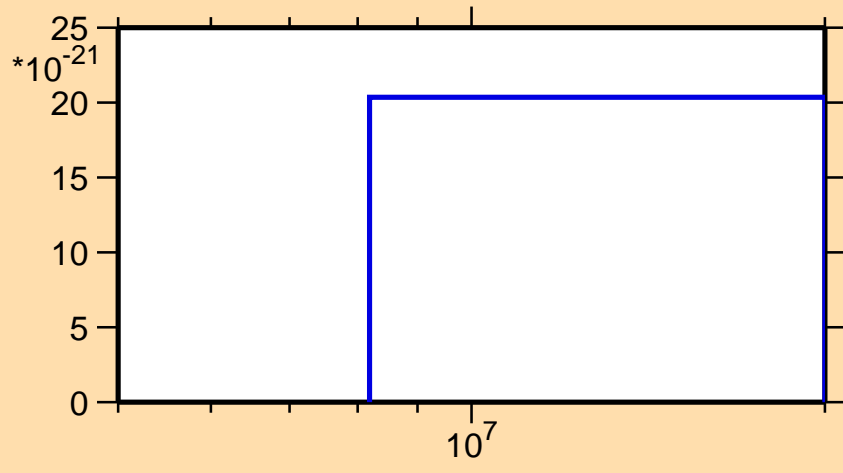
\sigma vs. E for ^{201}\text{At}(\text{mt } 42)
