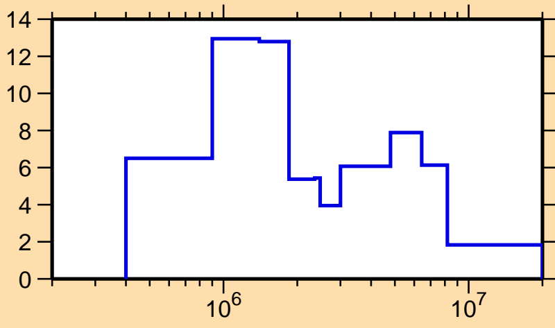
\Delta\sigma/\sigma vs. E for ^{201}\text{At}(n,\text{el.})
