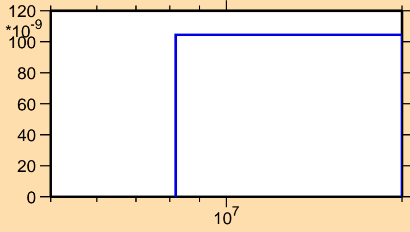
\sigma vs. E for ^{201}\text{At}(n,2n\alpha)
