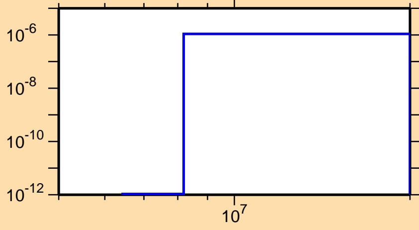
\sigma vs. E for ^{201}\text{At}(n,\text{He3})
