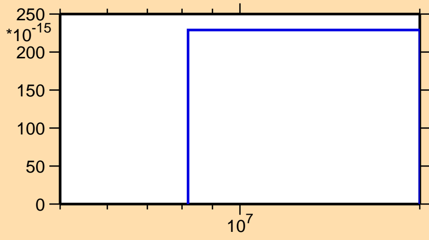
\sigma vs. E for ^{201}\text{At}(\text{mt } 34)
