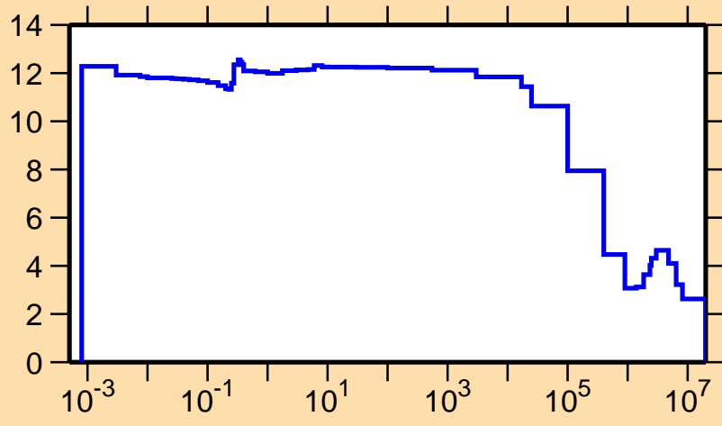
\sigma vs. E for ^{201}\text{At}(n,\text{el.})
