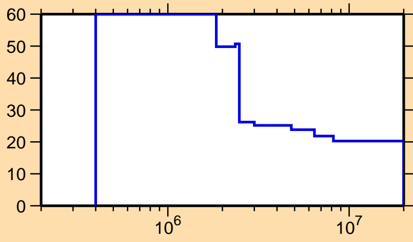
\Delta\sigma/\sigma vs. E for ^{201}\text{At}(n,n_1)
