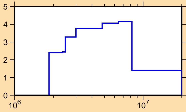
\Delta\sigma/\sigma vs. E for ^{201}\text{At}(n,\text{tot.})
