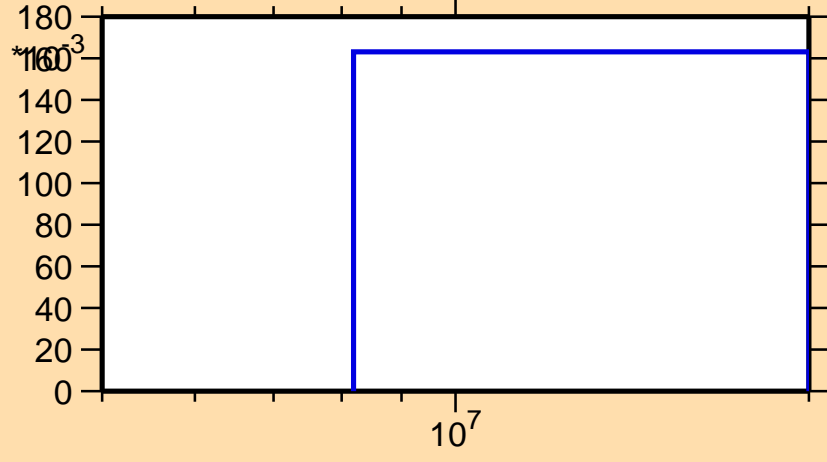
\sigma vs. E for ^{201}\text{At}(n,2n)
