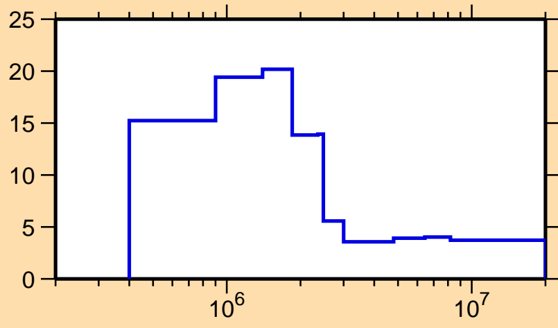
\Delta\sigma/\sigma vs. E for ^{201}\text{At}(n,\text{nonel.})
