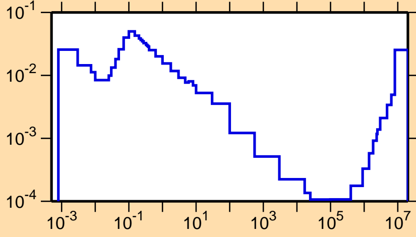
\sigma vs. E for ^{201}\text{At}(n,\alpha)
