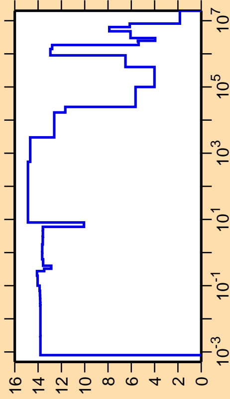
\Delta\sigma/\sigma vs. E for ^{201}\text{At}(n,\text{el.})
