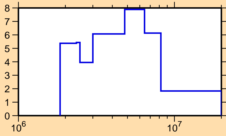
\Delta\sigma/\sigma vs. E for ^{201}\text{At}(n, \text{el.})
