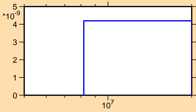
\sigma vs. E for ^{201}\text{At}(n,\text{pd})
