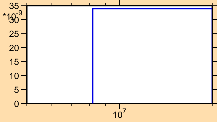
\sigma vs. E for ^{201}\text{At}(n,3n)
