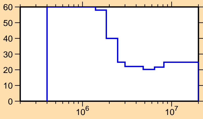
\Delta\sigma/\sigma vs. E for ^{201}\text{At}(n,\text{inel.})
