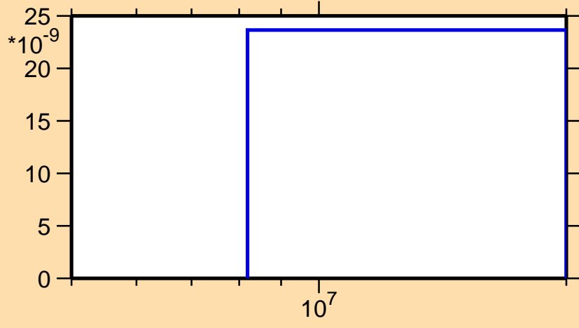
\sigma vs. E for ^{201}\text{At}(n,\text{nd})
