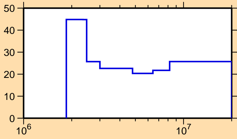
\Delta\sigma/\sigma vs. E for ^{201}\text{At}(n,n\text{cont.})
