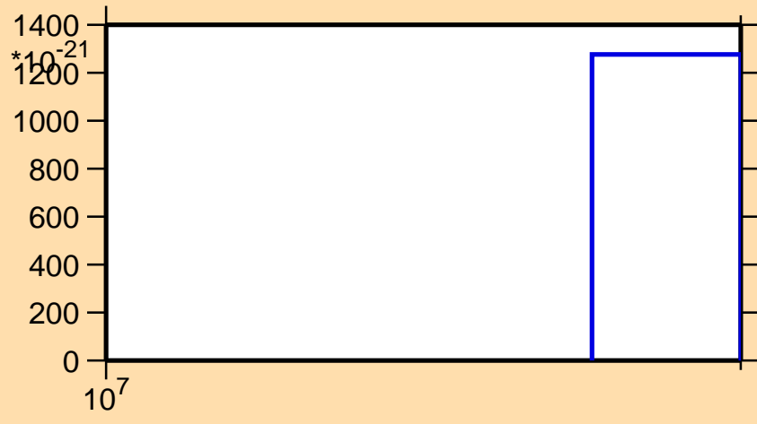
\sigma vs. E for ^{202}\text{At}(\text{mt } 42)
