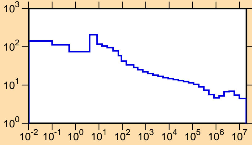
\sigma vs. E for ^{202}\text{At}(n,\text{tot.})
