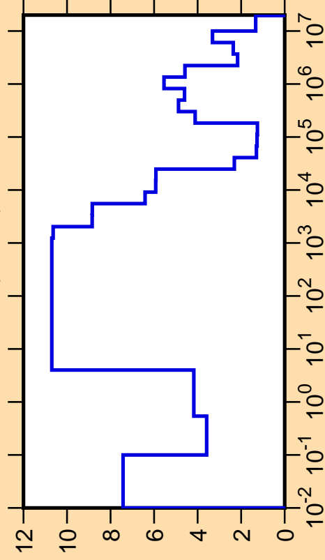
\Delta\sigma/\sigma vs. E for ^{202}\text{At}(n,\text{tot.})
