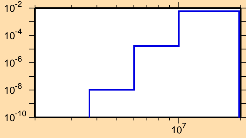
\sigma vs. E for ^{202}\text{At}(n,d)
