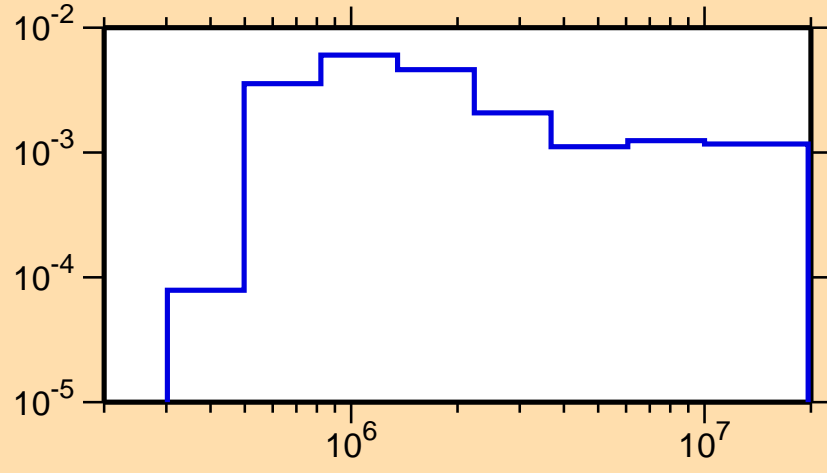
\sigma vs. E for ^{202}\text{At}(n,n_4)
