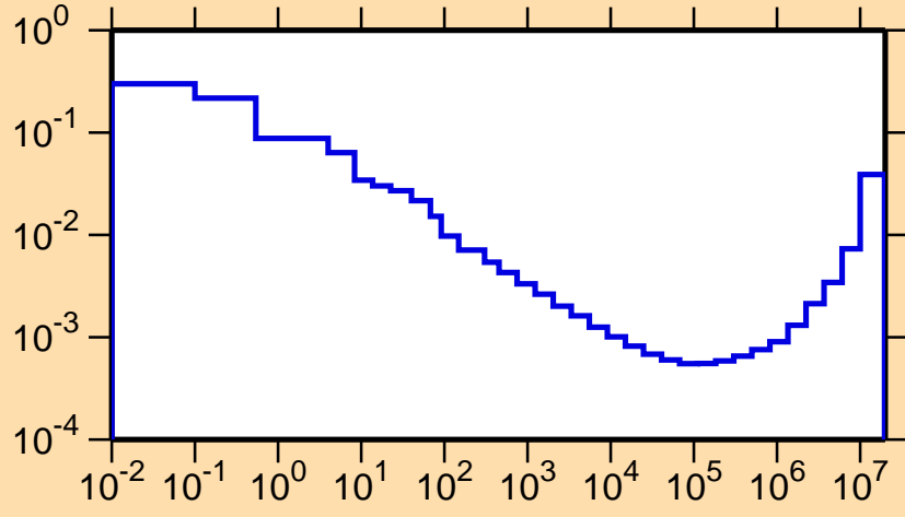
\sigma vs. E for ^{202}\text{At}(n,\alpha)
