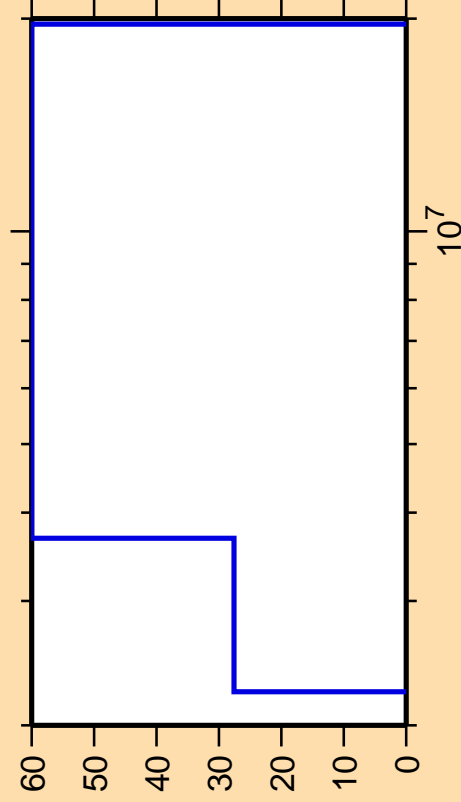
\Delta\sigma/\sigma vs. E for ^{202}\text{At}(n,d)
