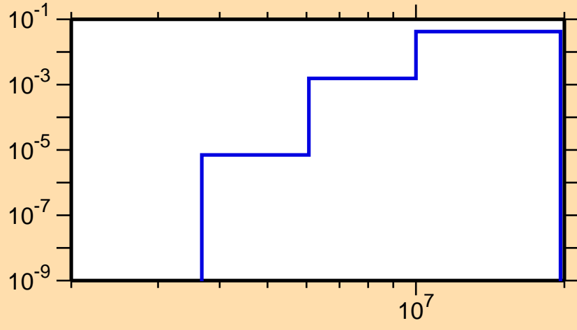
\sigma vs. E for ^{202}\text{At}(n,np)
