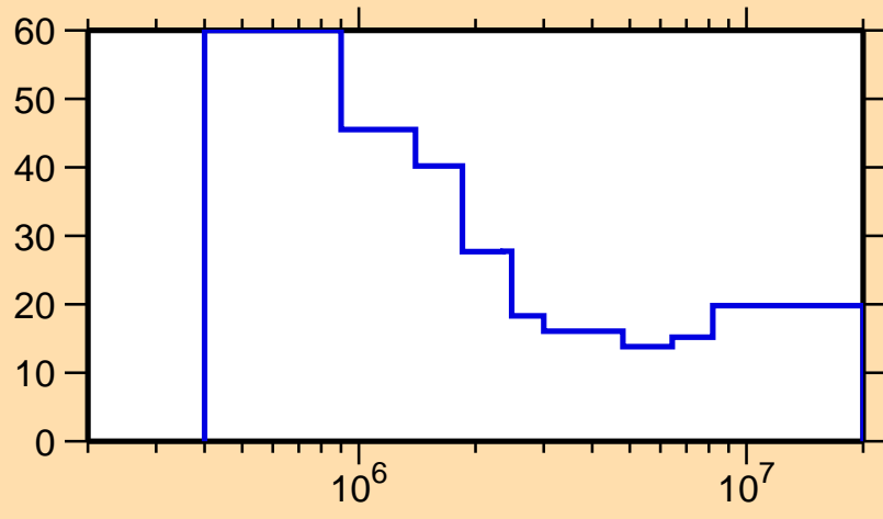
\Delta\sigma/\sigma vs. E for ^{202}\text{At}(n, ncont.)
