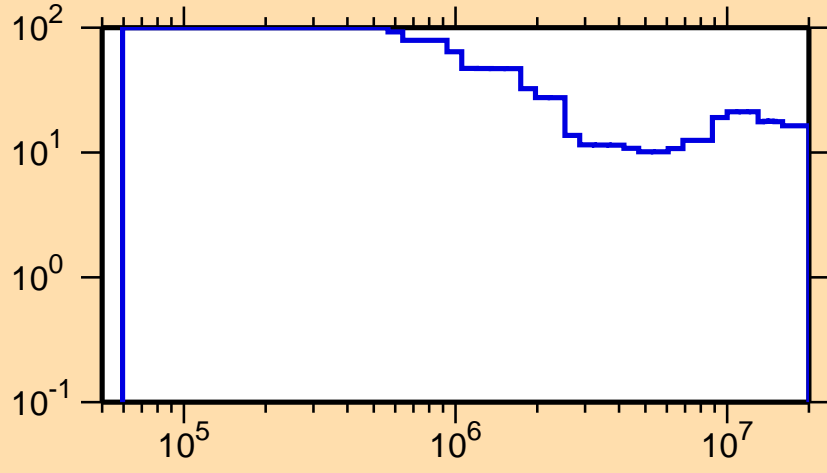
\Delta\sigma/\sigma vs. E for ^{202}\text{At}(n,ncont.)
