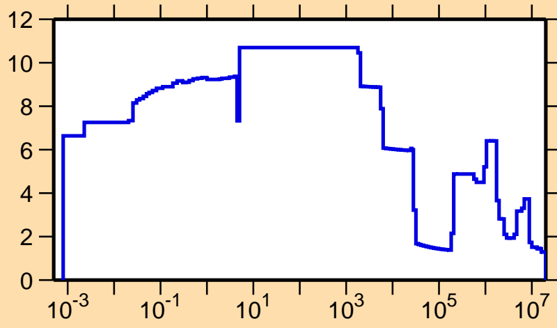
\Delta\sigma/\sigma vs. E for ^{202}\text{At}(n,\text{tot.})
