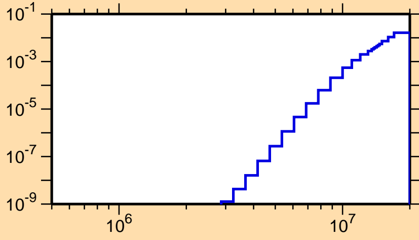
\sigma vs. E for ^{202}\text{At}(n,n\alpha)
