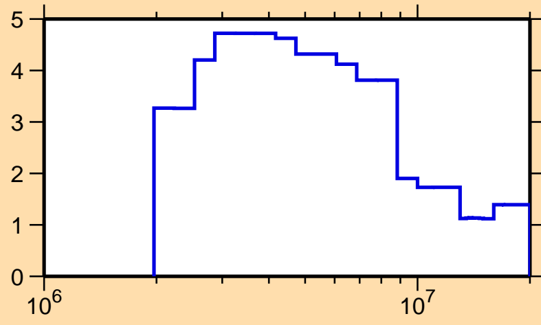
\Delta\sigma/\sigma vs. E for ^{203}\text{At}(n, tot.)
