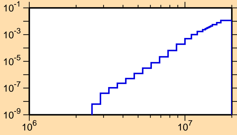
\sigma vs. E for ^{203}\text{At}(n,n\alpha)
