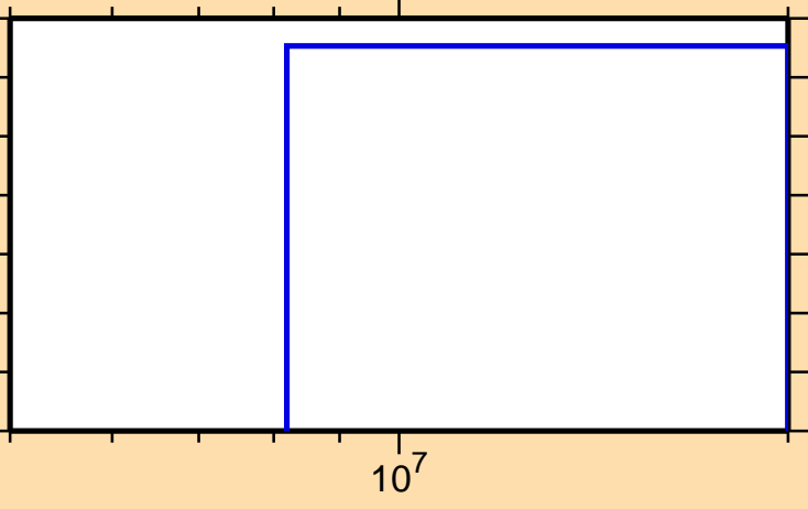
\sigma vs. E for ^{203}\text{At}(n,3n)
