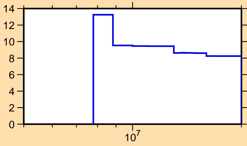
\Delta\sigma/\sigma vs. E for ^{204}\text{At}(n,2n)
