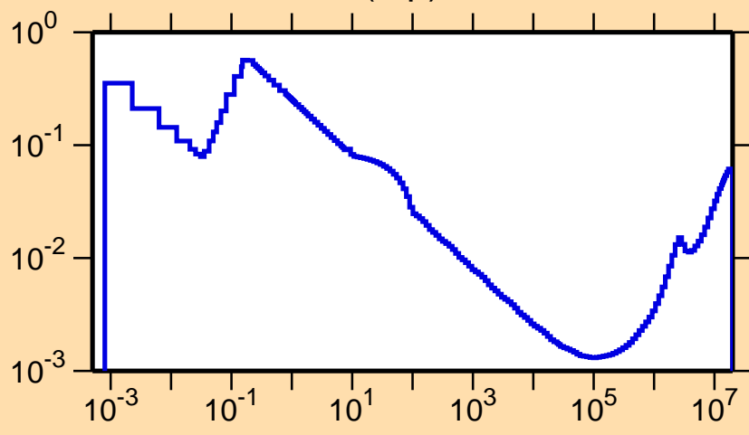
\sigma vs. E for ^{204}\text{At}(n,p)
