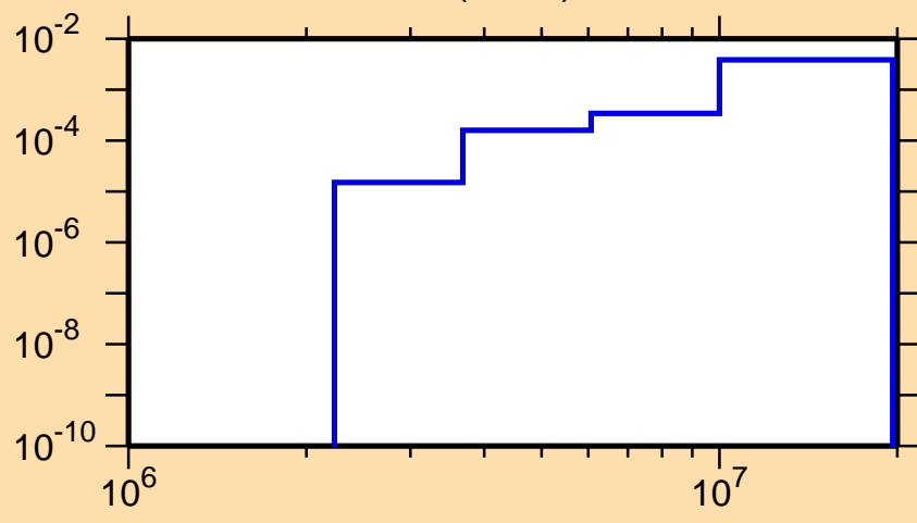
\sigma vs. E for ^{204}\text{At}(n,n\alpha)
