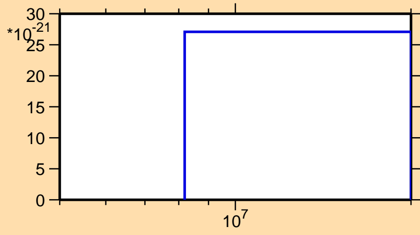
\sigma vs. E for ^{204}\text{At}(\text{mt } 42)
