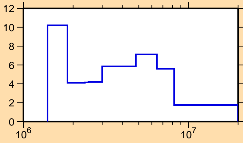
\Delta\sigma/\sigma vs. E for ^{204}\text{At}(n, el.)
