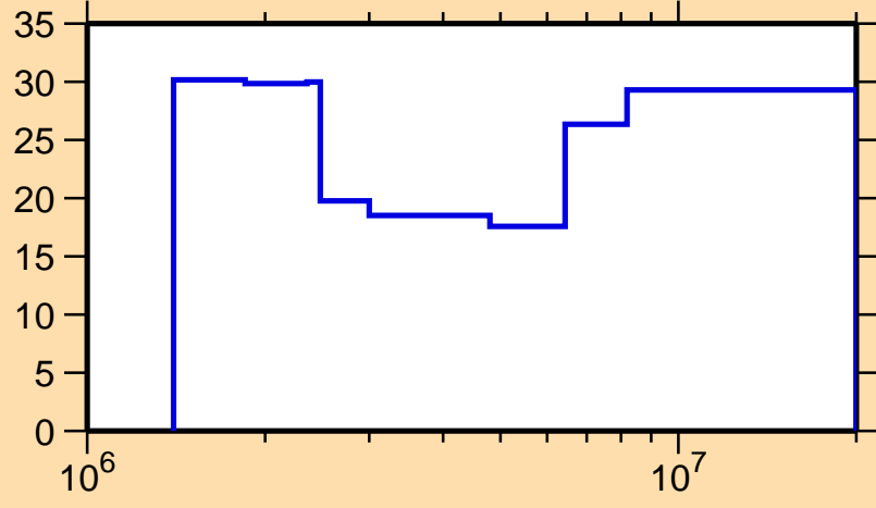
\Delta\sigma/\sigma vs. E for ^{204}\text{At}(n,n_1)
