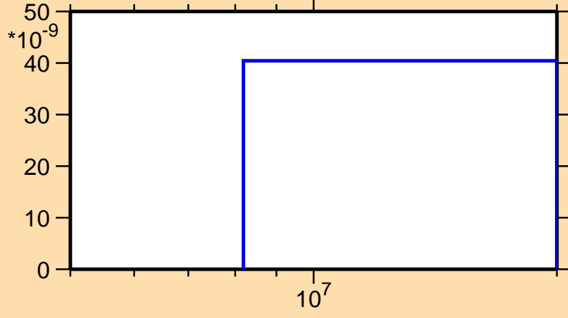
\sigma vs. E for ^{204}\text{At}(\text{mt117})
