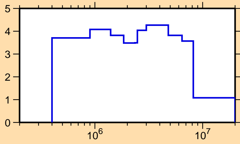
\Delta\sigma/\sigma vs. E for ^{204}\text{At}(n,\text{tot.})
