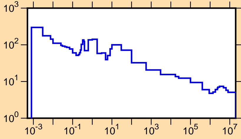
\sigma vs. E for ^{204}\text{At}(n,\text{tot.})
