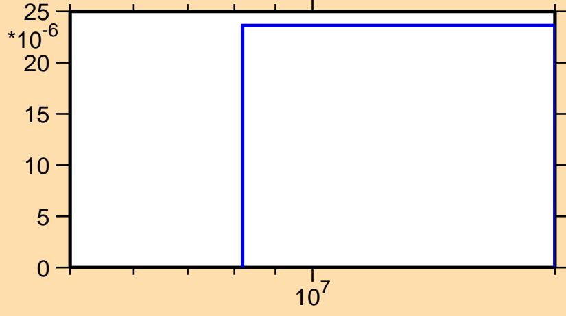
\sigma vs. E for ^{204}\text{At}(n,2np)
