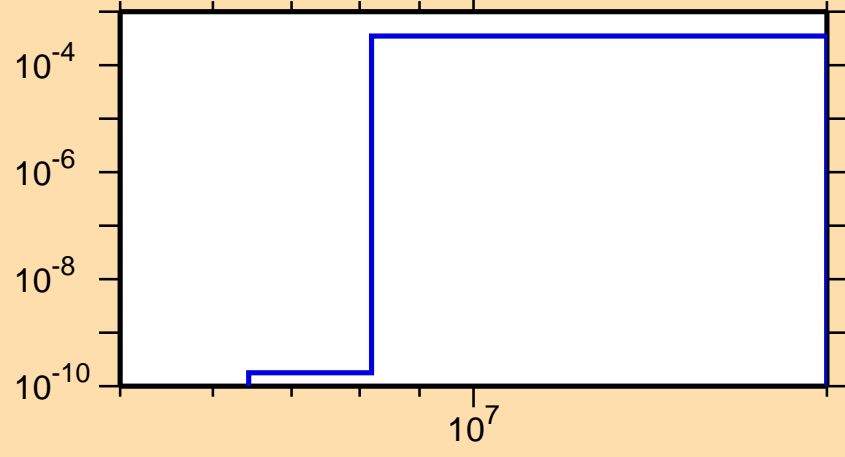
\sigma vs. E for ^{204}\text{At}(n,t)
