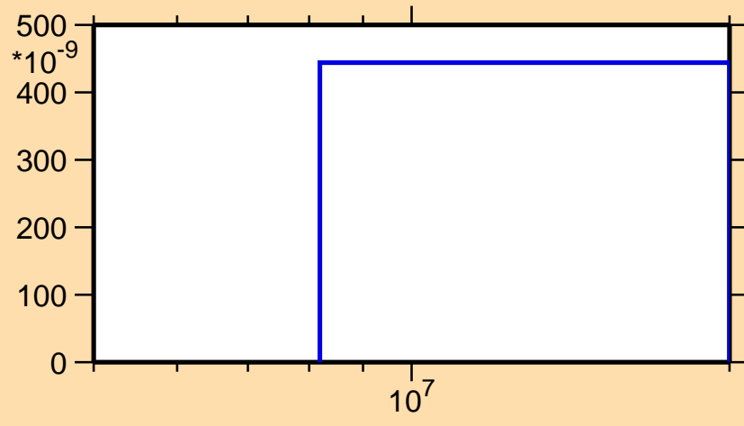
\sigma vs. E for ^{204}\text{At}(\text{mt } 45)
