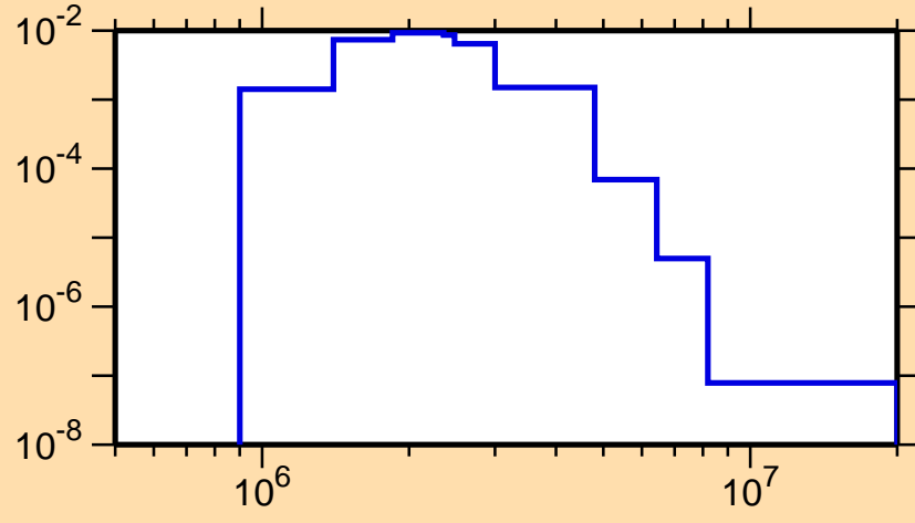
\sigma vs. E for ^{204}\text{At}(n,n_3)
