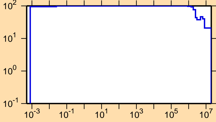
\Delta\sigma/\sigma vs. E for ^{204}\text{At}(n,p)
