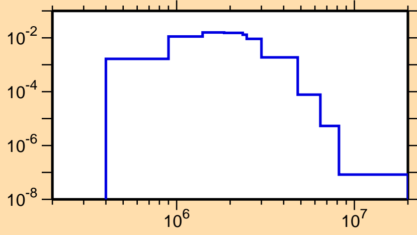
\sigma vs. E for ^{204}\text{At}(n,n_1)
