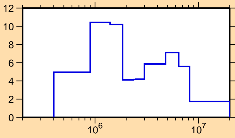
\Delta\sigma/\sigma vs. E for ^{204}\text{At}(n,\text{el.})
