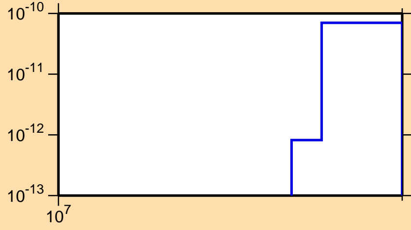
\sigma vs. E for ^{205}\text{At}(n,pt)
