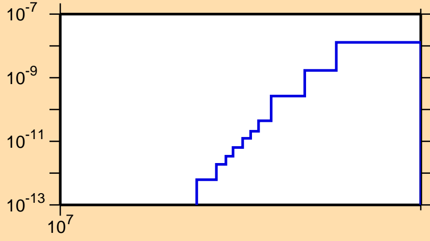
\sigma vs. E for ^{205}\text{At}(n,\text{pd})
