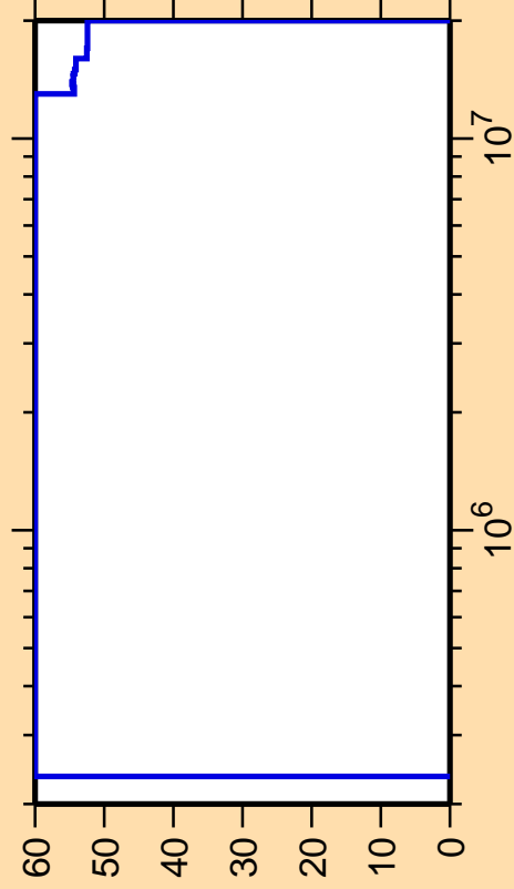
\Delta\sigma/\sigma vs. E for ^{205}\text{At}(n,\alpha)
