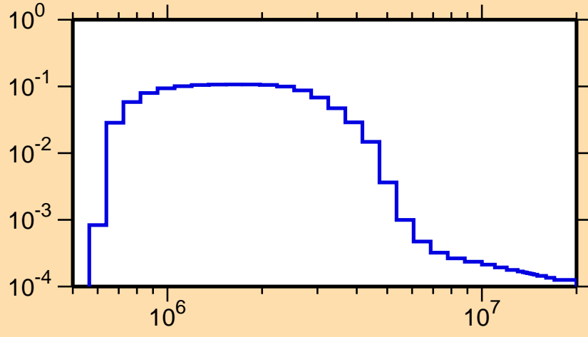
\sigma vs. E for ^{205}\text{At}(n,n_2)
