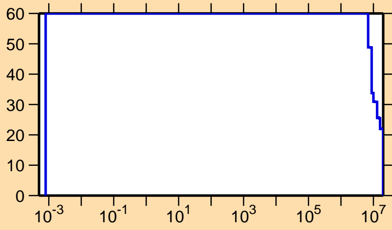
\Delta\sigma/\sigma vs. E for ^{205}\text{At}(n,p)
