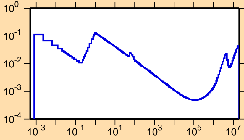
\sigma vs. E for ^{205}\text{At}(n,p)
