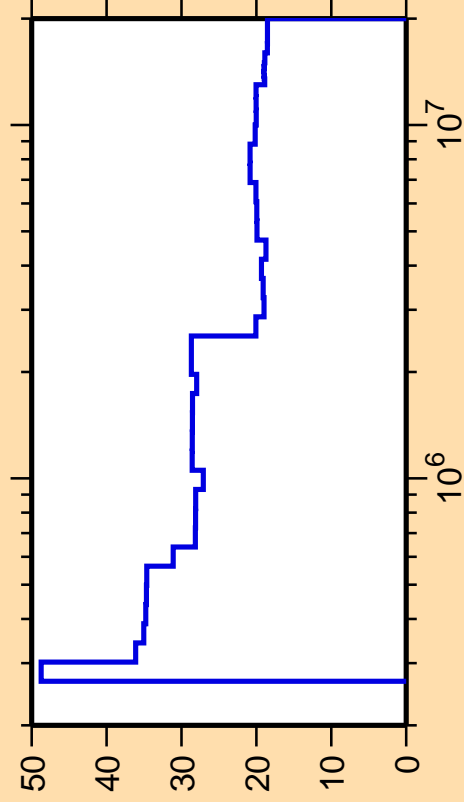
\Delta\sigma/\sigma vs. E for ^{205}\text{At}(n,n_1)
