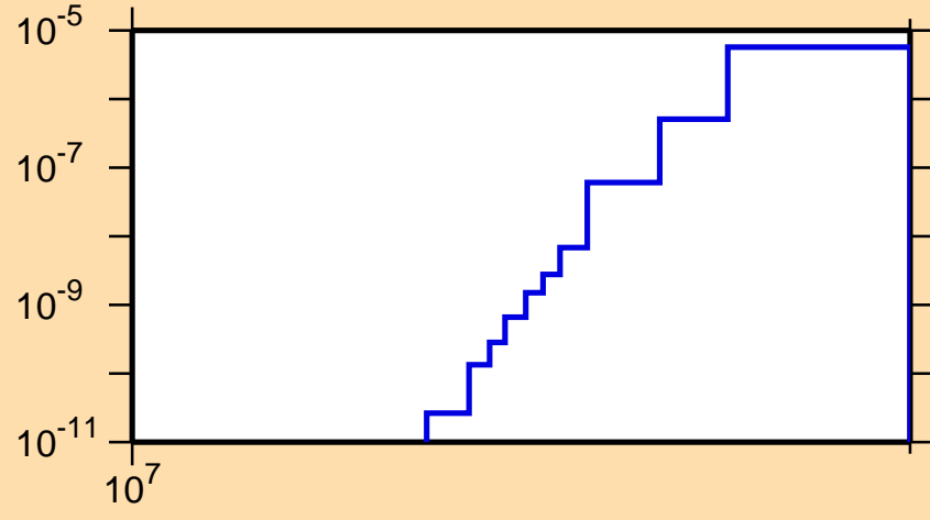
\sigma vs. E for ^{205}\text{At}(n,\text{nd})
