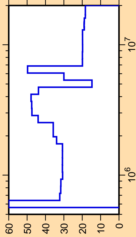
\Delta\sigma/\sigma vs. E for ^{205}\text{At}(n,n_2)
