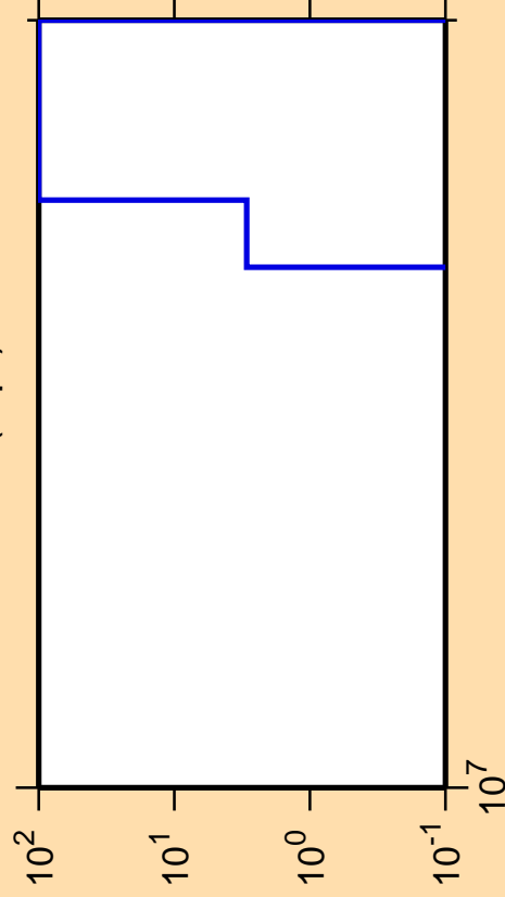
\Delta\sigma/\sigma vs. E for ^{205}\text{At}(n,pt)
