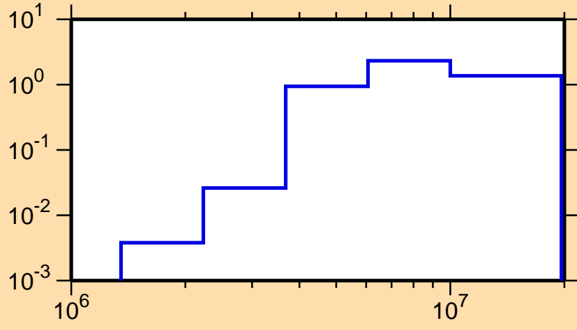
\sigma vs. E for ^{205}\text{At}(n,n\text{cont.})
