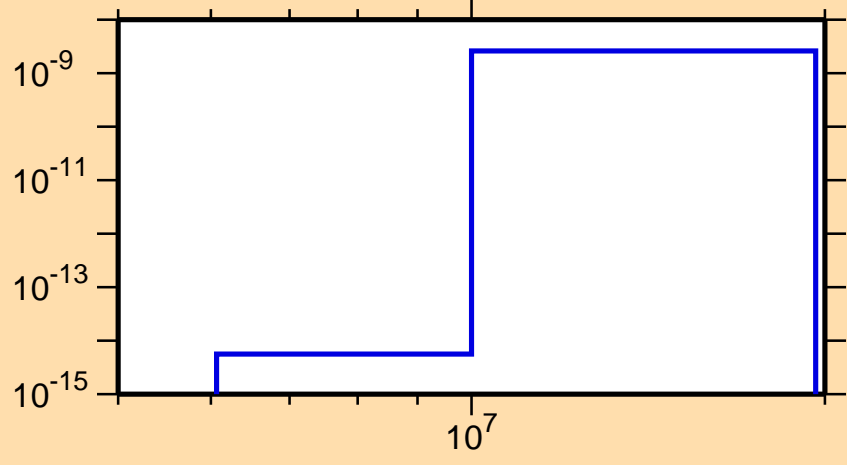
\sigma vs. E for ^{205}\text{At}(mt\ 45)
