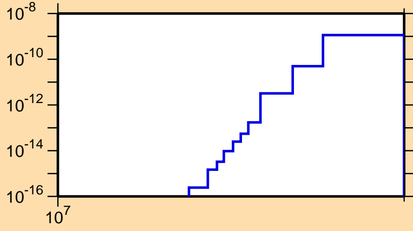
\sigma vs. E for ^{206}\text{At}(n,pt)
