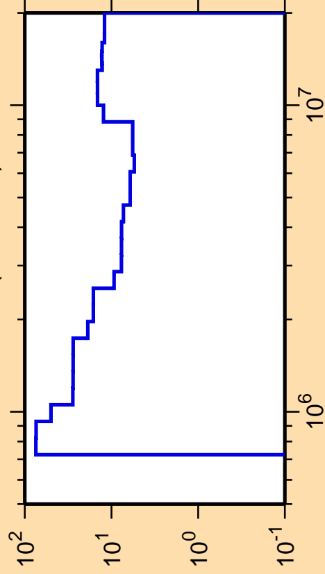
\Delta\sigma/\sigma vs. E for ^{206}\text{At}(n,\text{ncont.})
