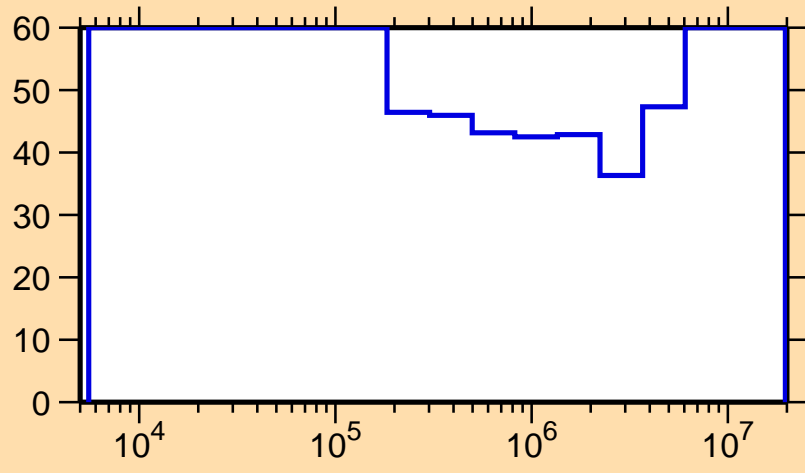
\Delta\sigma/\sigma vs. E for ^{206}\text{At}(n,n_1)
