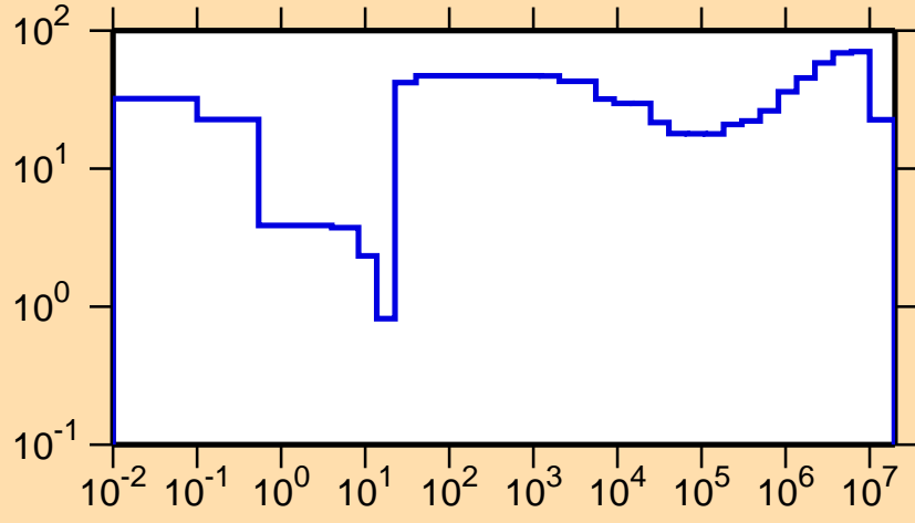
\Delta\sigma/\sigma vs. E for ^{206}\text{At}(n,\gamma)
