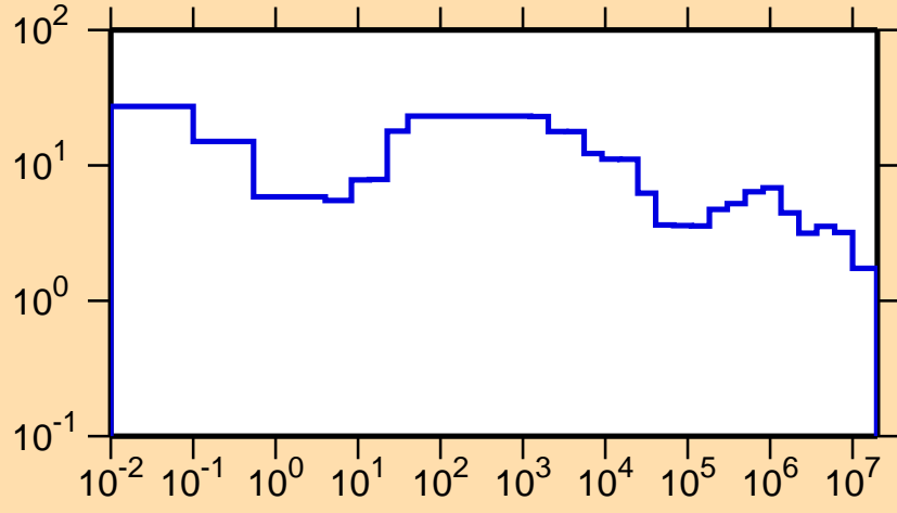
\Delta\sigma/\sigma vs. E for ^{206}\text{At}(n,\text{tot.})
