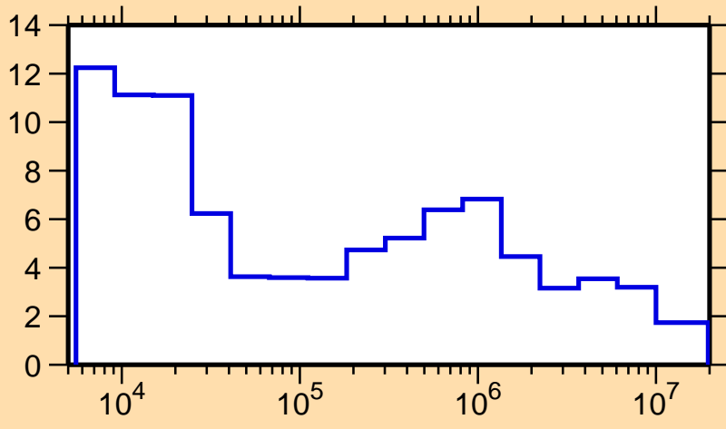
\Delta\sigma/\sigma vs. E for ^{206}\text{At}(n,\text{tot.})
