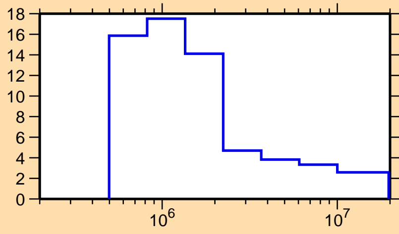
\Delta\sigma/\sigma vs. E for ^{206}\text{At}(n,\text{nonel.})
