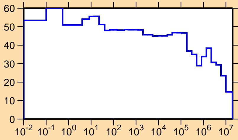
\Delta\sigma/\sigma vs. E for ^{206}\text{At}(n,p)
