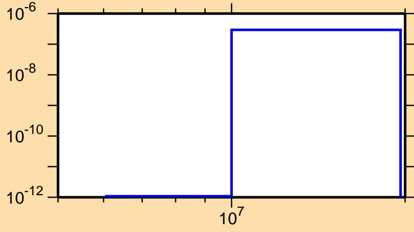
\sigma vs. E for ^{206}\text{At}(n,\text{He3})
