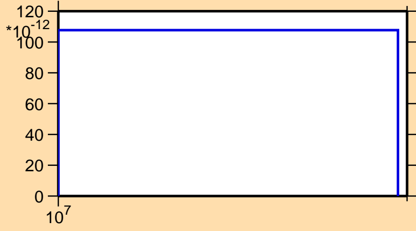
\sigma vs. E for ^{206}\text{At}(\text{mt117})
