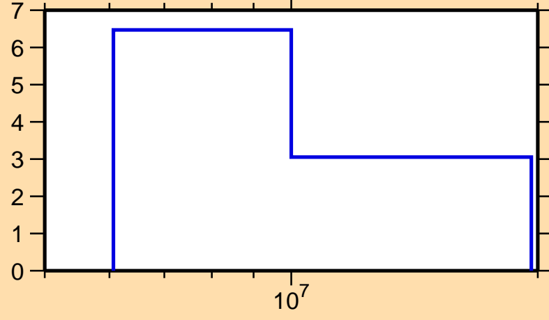
\Delta\sigma/\sigma vs. E for ^{206}\text{At}(n,\text{el.})
