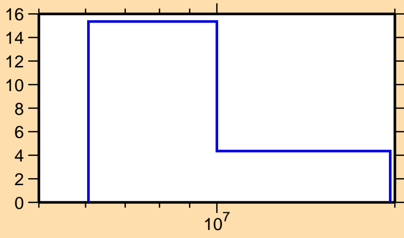
\Delta\sigma/\sigma vs. E for ^{206}\text{At}(n,2n)
