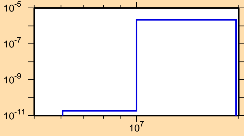
\sigma vs. E for ^{206}\text{At}(n,2n\alpha)
