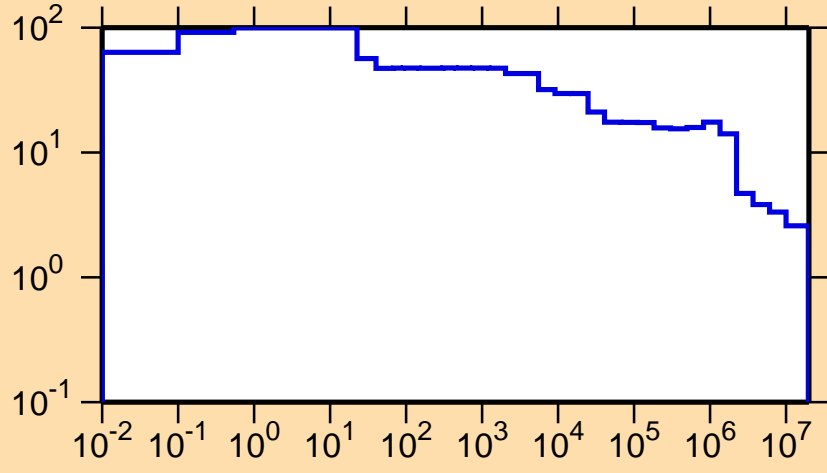
\Delta\sigma/\sigma vs. E for ^{206}\text{At}(n,\text{nonel.})
