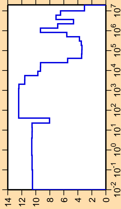
\Delta\sigma/\sigma vs. E for ^{206}\text{At}(n,\text{el.})
