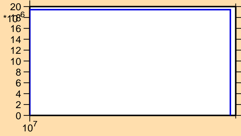
\sigma vs. E for ^{206}\text{At}(n,3n)
