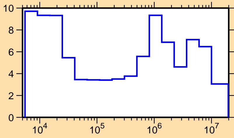
\Delta\sigma/\sigma vs. E for ^{206}\text{At}(n,\text{el.})
