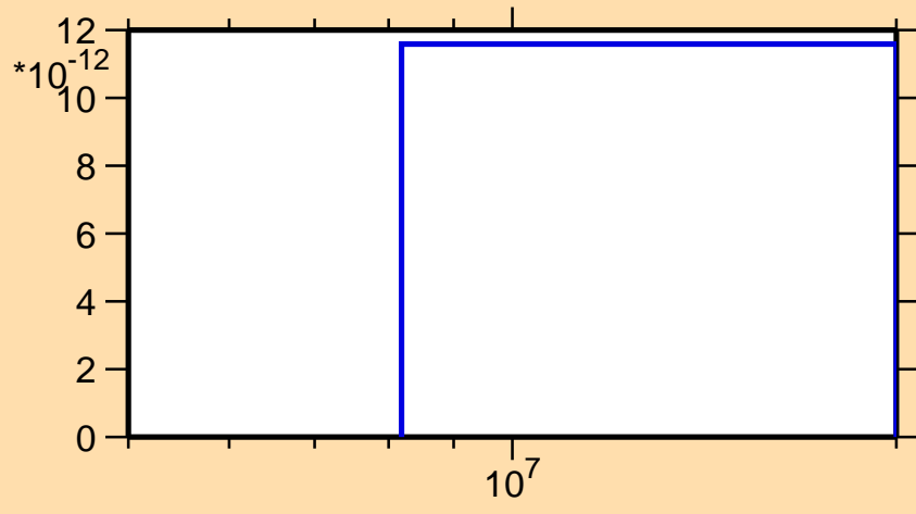
\sigma vs. E for ^{206}\text{At}(n,\text{pt})
