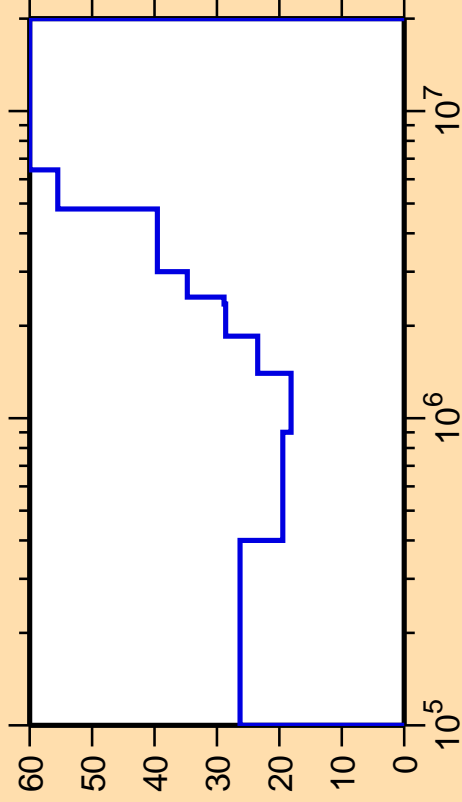
\Delta\sigma/\sigma vs. E for ^{206}\text{At}(n,n_4)
