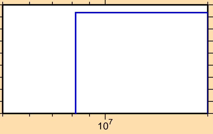
\sigma vs. E for ^{206}\text{At}(n,3n)
