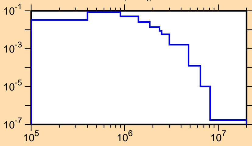
\sigma vs. E for ^{206}\text{At}(n,n_4)
