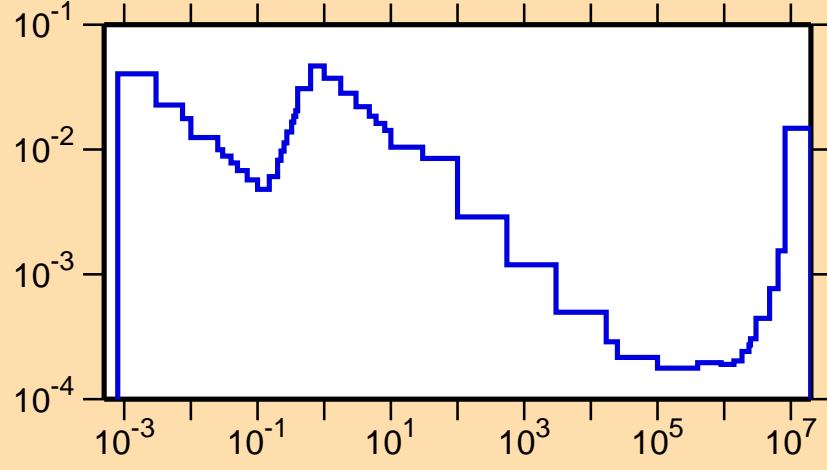
\sigma vs. E for ^{206}\text{At}(n,\alpha)
