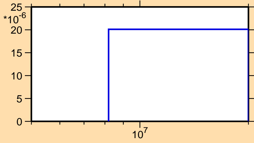
\sigma vs. E for ^{206}\text{At}(n,2np)
