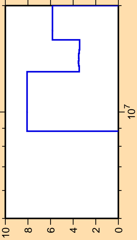
\Delta\sigma/\sigma vs. E for ^{207}\text{At}(n,2n)
