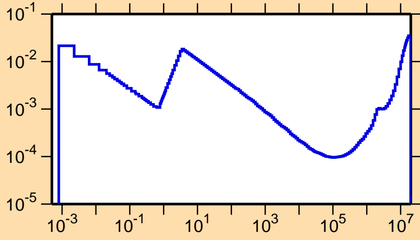
\sigma vs. E for ^{207}\text{At}(n,p)
