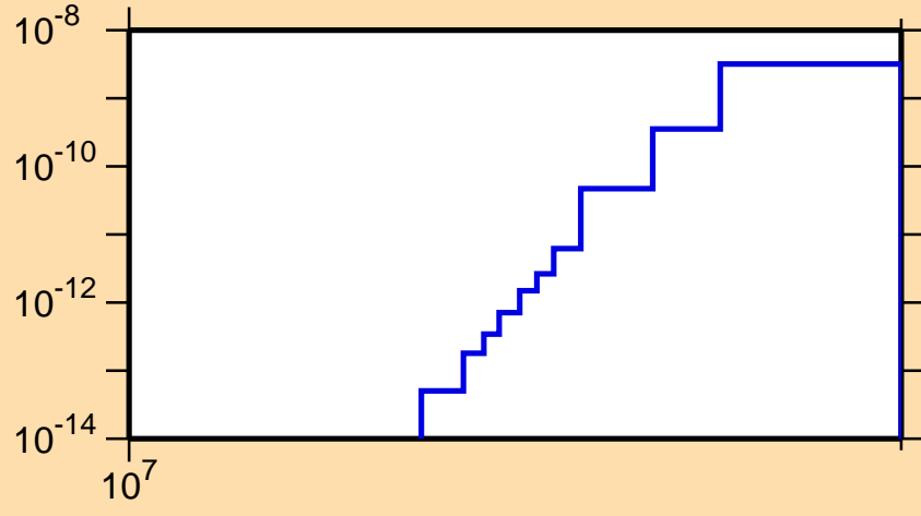
\sigma vs. E for ^{207}\text{At}(n,\text{pd})
