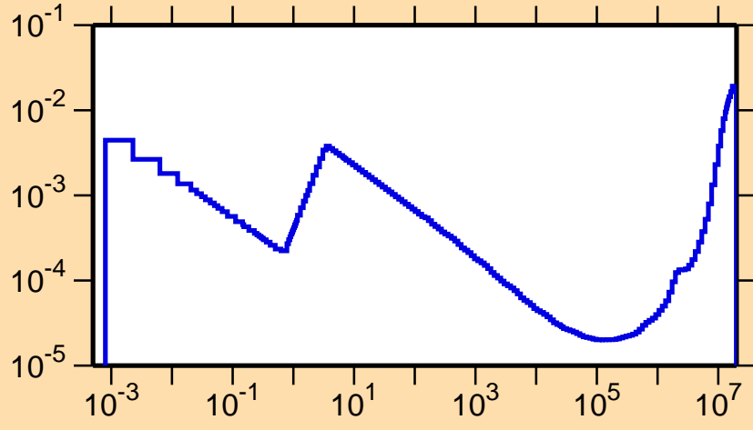
\sigma vs. E for ^{207}\text{At}(n,\alpha)
