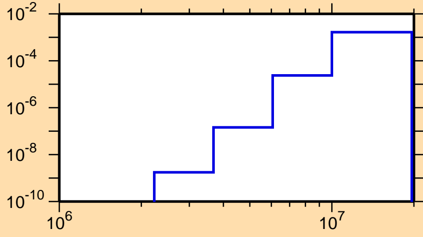
\sigma vs. E for ^{207}\text{At}(n,n\alpha)
