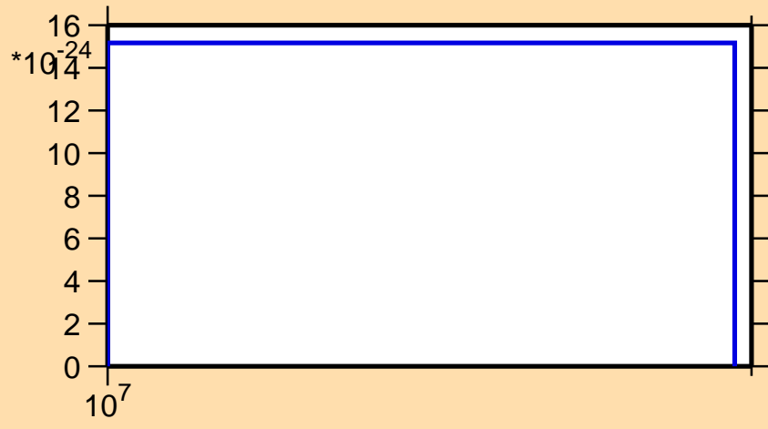
\sigma vs. E for ^{207}\text{At}(\text{mt } 42)
