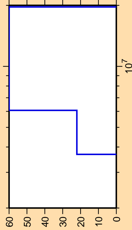
\Delta\sigma/\sigma vs. E for ^{207}\text{At}(n,p\alpha)
