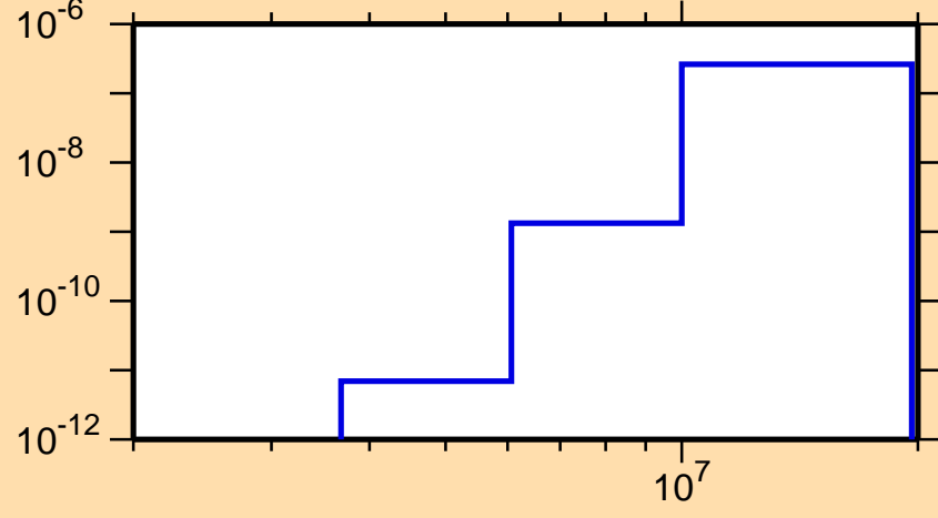
\sigma vs. E for ^{207}\text{At}(n,p\alpha)
