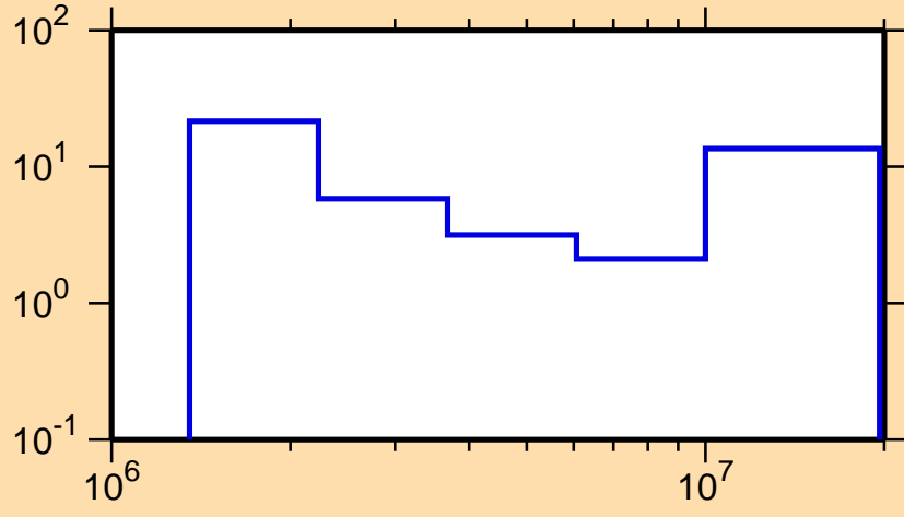
\Delta\sigma/\sigma vs. E for ^{207}\text{At}(n,ncont.)
