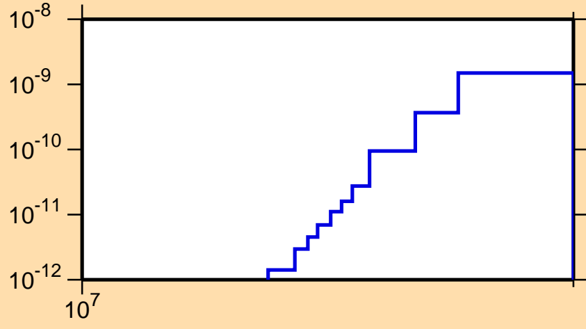
\sigma vs. E for ^{208}\text{At}(\text{mt117})
