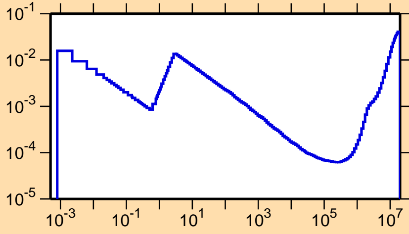
\sigma vs. E for ^{208}\text{At}(n,p)
