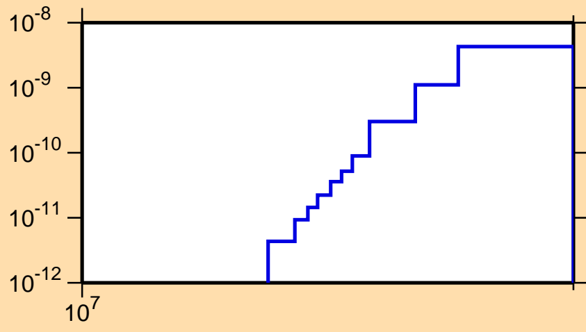
\sigma vs. E for ^{208}\text{At}(\text{mt } 45)
