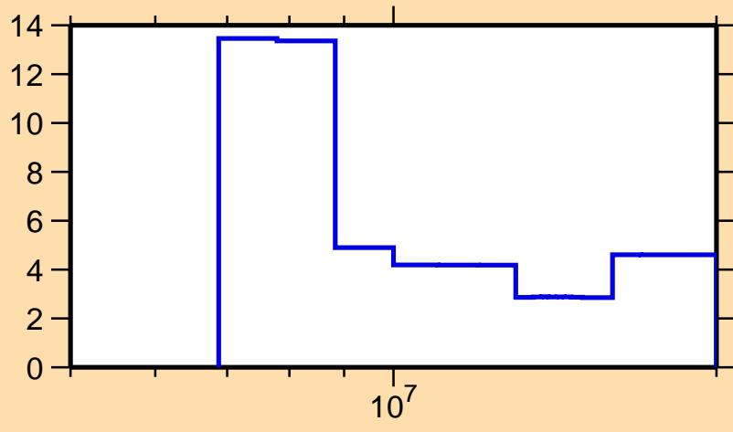
\Delta\sigma/\sigma vs. E for ^{208}\text{At}(n,2n)
