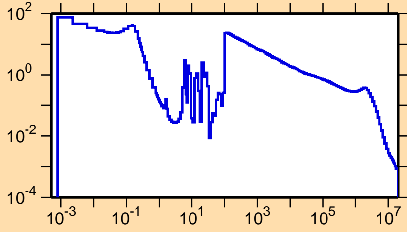
\sigma vs. E for ^{208}\text{At}(n,\gamma)
