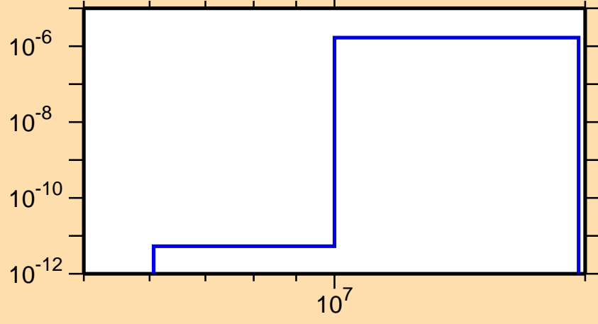
\sigma vs. E for ^{208}\text{At}(n,2n\alpha)
