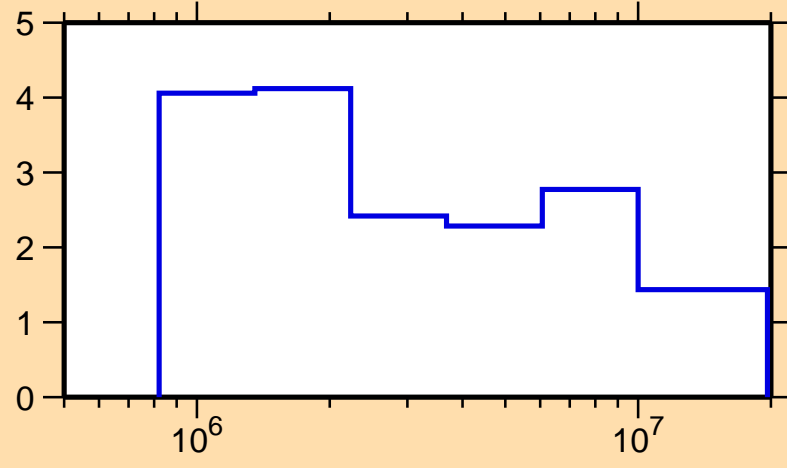
\Delta\sigma/\sigma vs. E for ^{208}\text{At}(n,\text{tot.})
