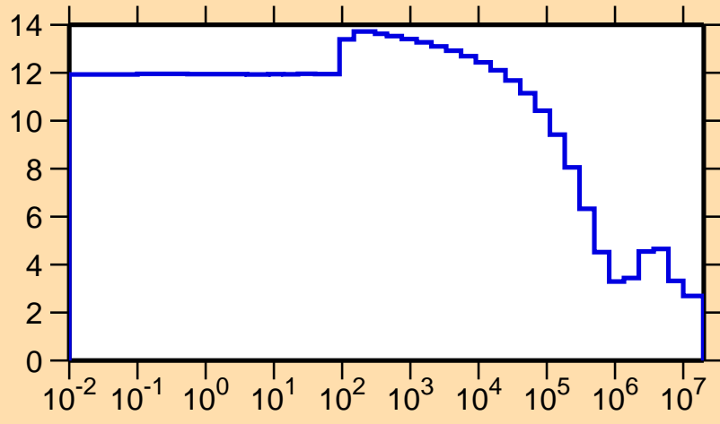
\sigma vs. E for ^{208}\text{At}(n,\text{el.})
