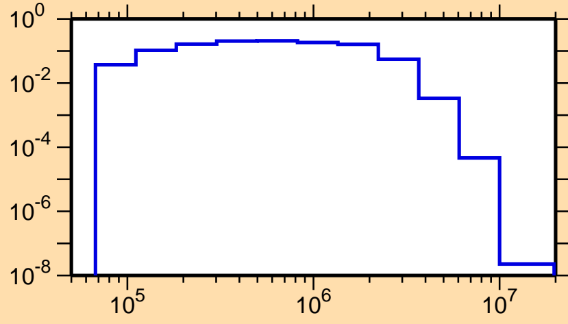
\sigma vs. E for ^{208}\text{At}(n,n_3)
