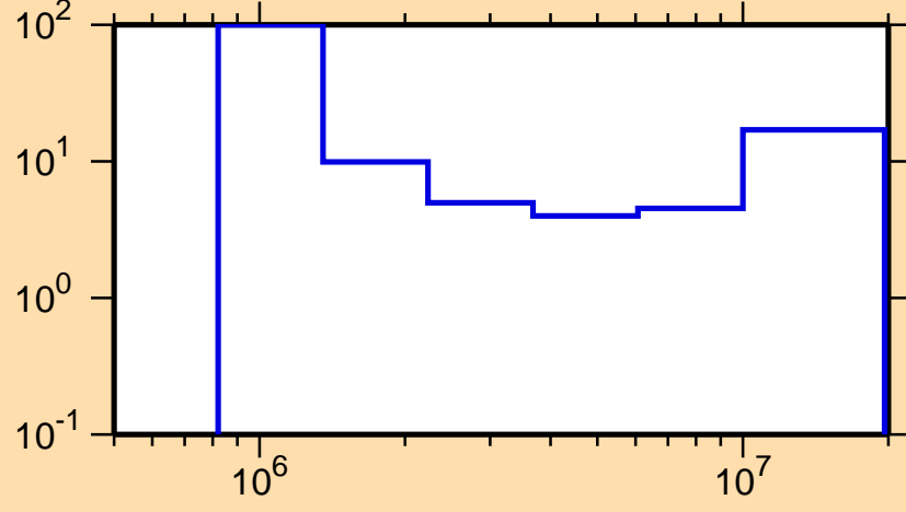
\Delta\sigma/\sigma vs. E for ^{208}\text{At}(n,n\text{cont.})
