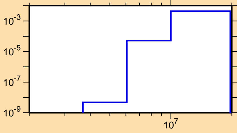
\sigma vs. E for ^{208}\text{At}(n,np)
