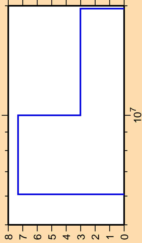
\Delta\sigma/\sigma vs. E for ^{208}\text{At}(n,2n)
