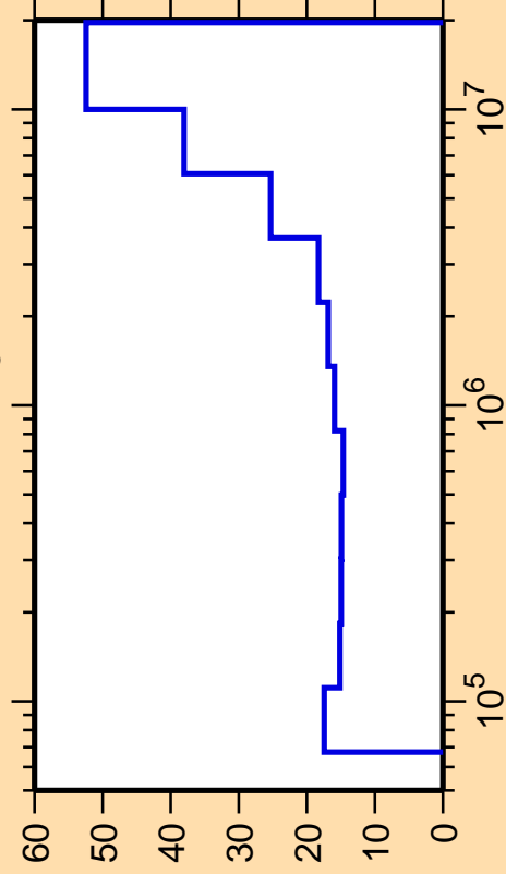
\Delta\sigma/\sigma vs. E for ^{208}\text{At}(n,n_3)
