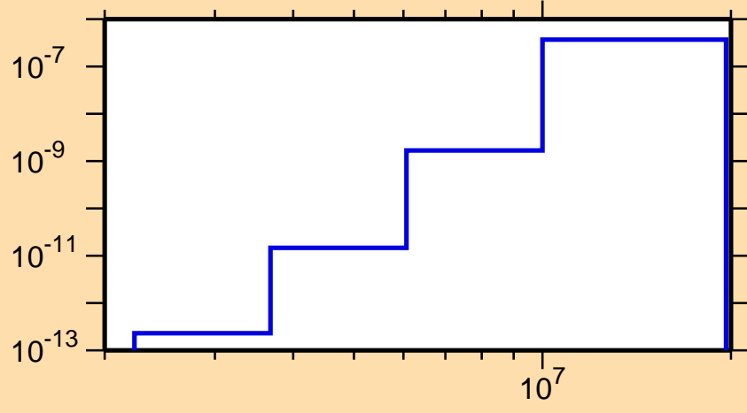
\sigma vs. E for ^{208}\text{At}(n,p\alpha)
