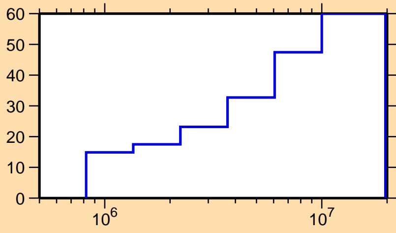
\Delta\sigma/\sigma vs. E for ^{208}\text{At}(n,n_1)
