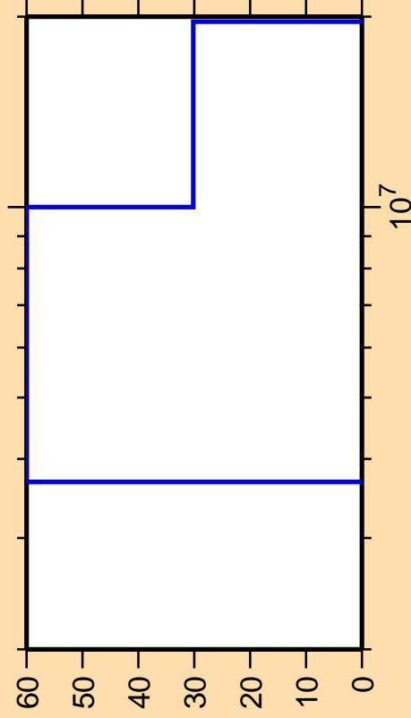
\Delta\sigma/\sigma vs. E for ^{208}\text{At}(n,np)
