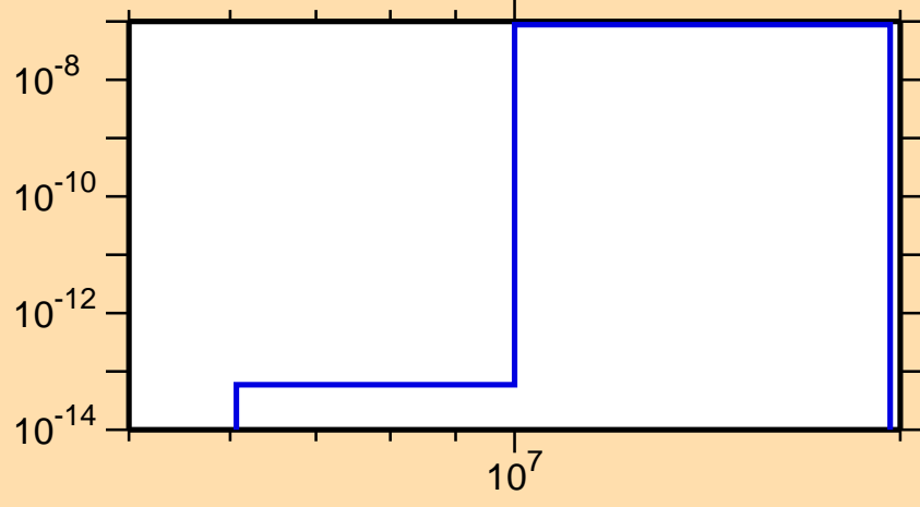
\sigma vs. E for ^{208}\text{At}(n,\text{He3})
