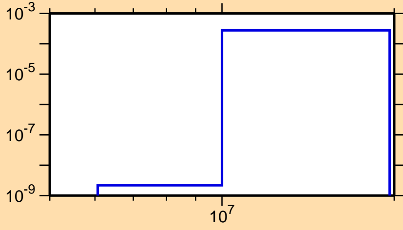
\sigma vs. E for ^{208}\text{At}(n,t)
