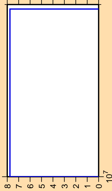
\Delta\sigma/\sigma vs. E for ^{208}\text{At}(\text{mt } 34)
