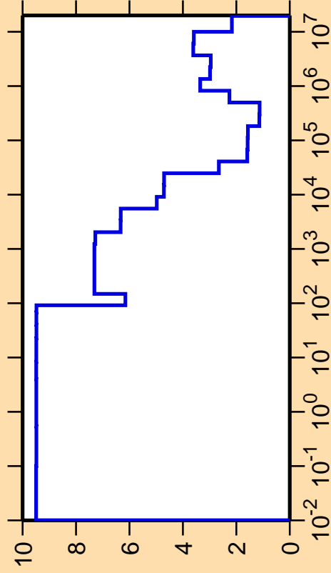
\Delta\sigma/\sigma vs. E for ^{208}\text{At}(n,\text{el.})
