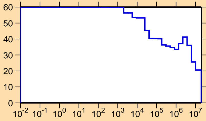
\Delta\sigma/\sigma vs. E for ^{208}\text{At}(n,p)
