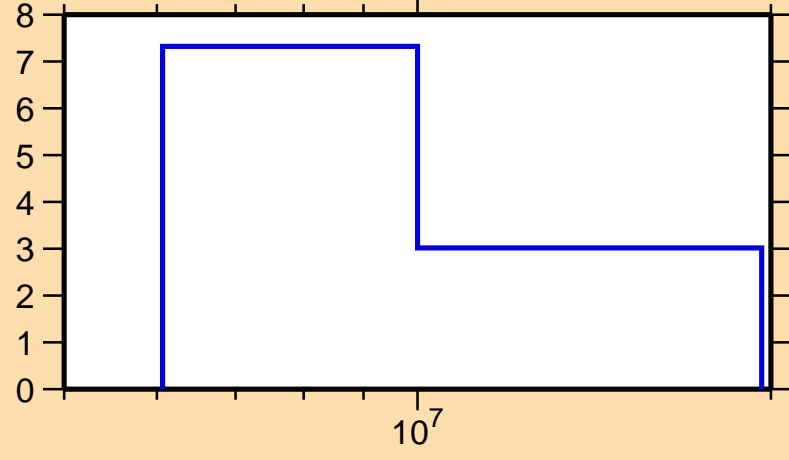
\Delta\sigma/\sigma vs. E for ^{208}\text{At}(n,2n)
