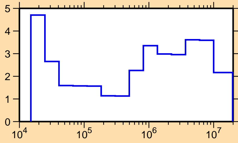
\Delta\sigma/\sigma vs. E for ^{208}\text{At}(n,\text{el.})
