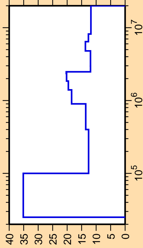
\Delta\sigma/\sigma vs. E for ^{208}\text{At}(n,n_2)
