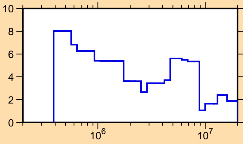
\Delta\sigma/\sigma vs. E for ^{209}\text{At}(n,\text{el.})
