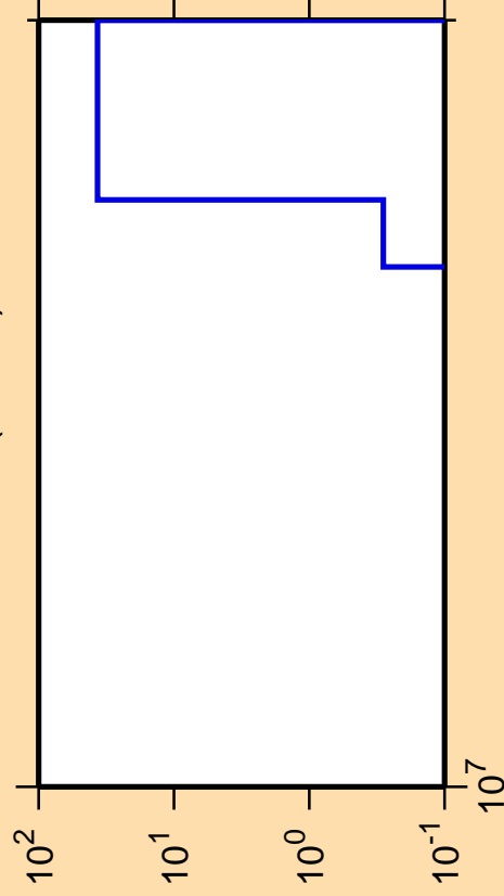
\Delta\sigma/\sigma vs. E for ^{209}\text{At}(\text{mt } 34)
