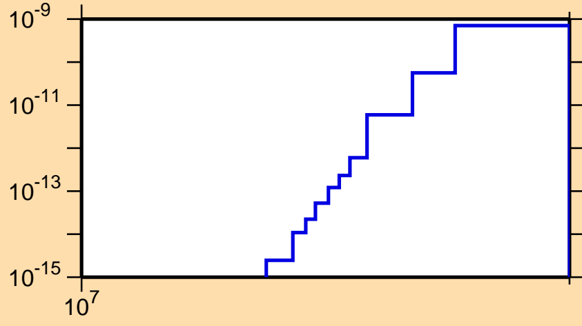
\sigma vs. E for ^{209}\text{At}(n,\text{pd})
