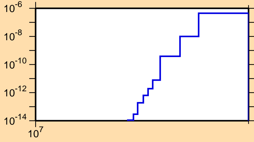
\sigma vs. E for ^{209}\text{At}(n,nt)
