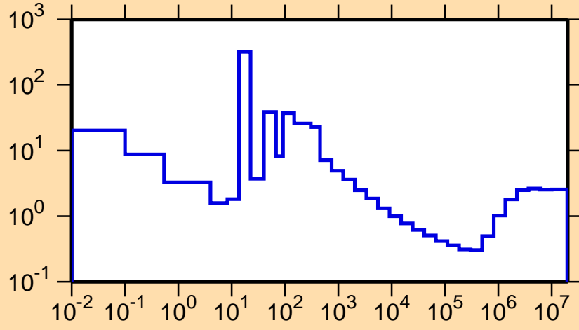
\sigma vs. E for ^{209}\text{At}(n,\text{nonel.})
