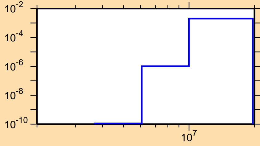
\sigma vs. E for ^{209}\text{At}(n,d)
