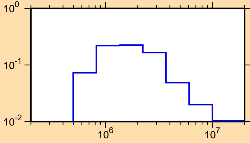
\sigma vs. E for ^{209}\text{At}(n,n_2)
