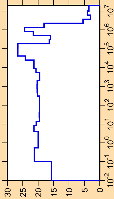
\Delta\sigma/\sigma vs. E for ^{209}\text{At}(n,\text{nonel.})
