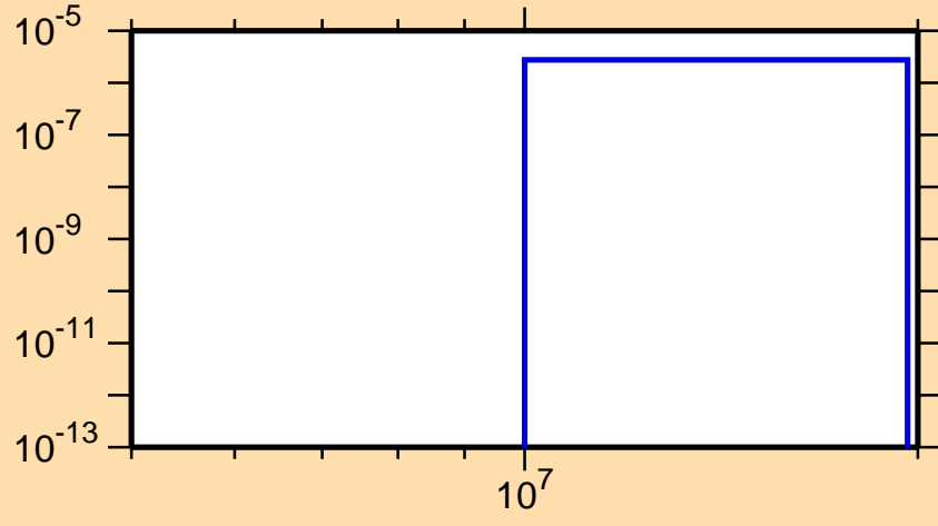
\sigma vs. E for ^{218}\text{At}(n,\text{nd})
