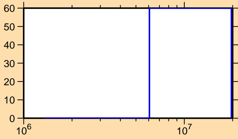
\Delta\sigma/\sigma vs. E for ^{218}\text{At}(n,f)
