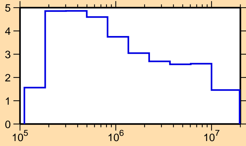
\sigma vs. E for ^{218}\text{At}(n,\text{inel.})
