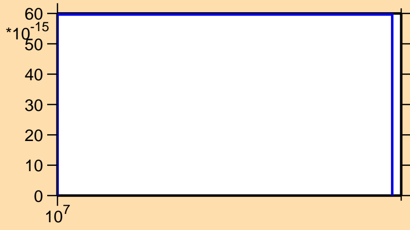
\sigma vs. E for ^{218}\text{At}(\text{mt } 42)
