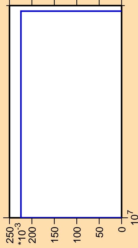
\Delta\sigma/\sigma vs. E for ^{218}\text{At}(\text{mt } 42)
