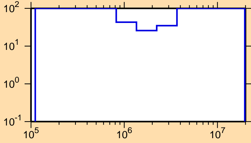
\Delta\sigma/\sigma vs. E for ^{218}\text{At}(n, ncont.)
