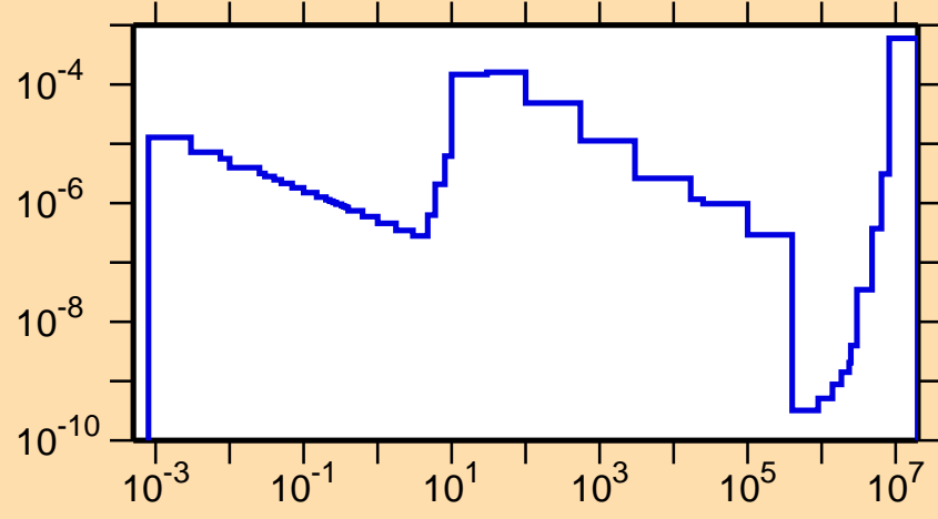
\sigma vs. E for ^{218}\text{At}(n,\alpha)
