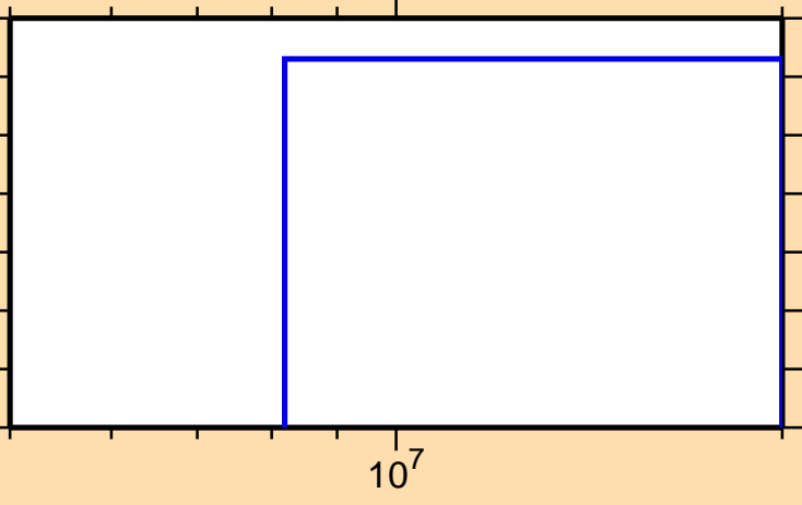
\sigma vs. E for ^{218}\text{At}(n,nt)
