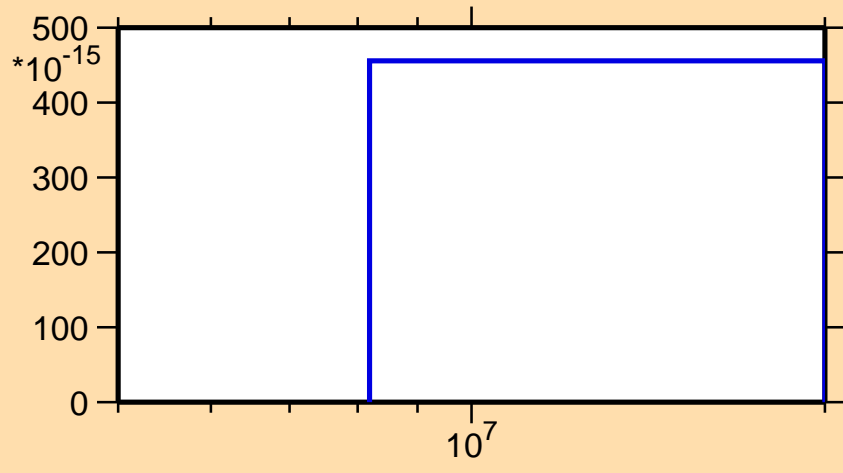
\sigma vs. E for ^{218}\text{At}(\text{mt } 34)
