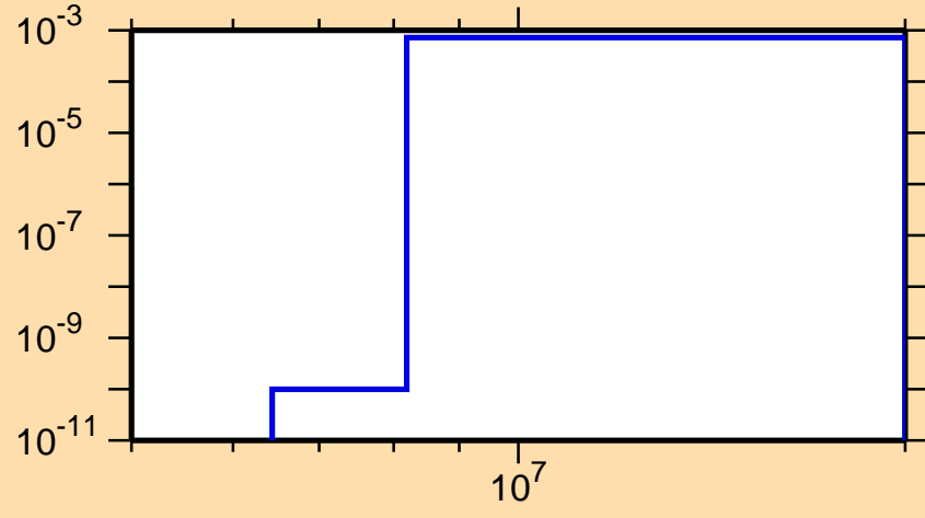
\sigma vs. E for ^{218}\text{At}(n,d)
