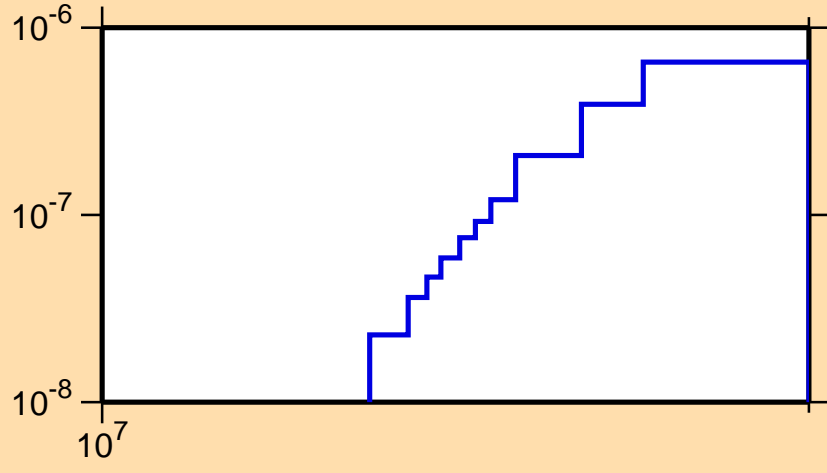
\sigma vs. E for ^{219}\text{At}(\text{mt117})
