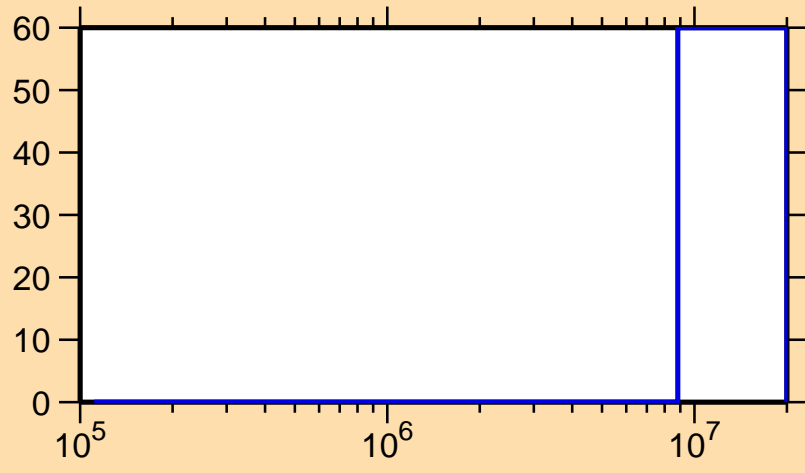
\Delta\sigma/\sigma vs. E for ^{219}\text{At}(n,f)
