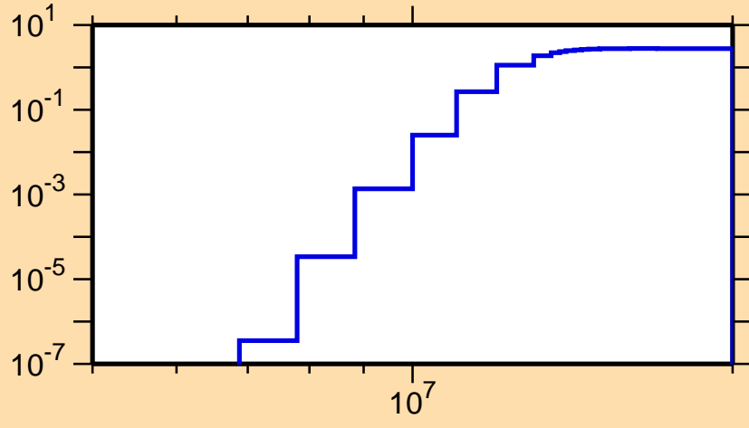
\sigma vs. E for ^{219}\text{At}(n,t)
