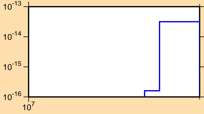
\sigma vs. E for ^{219}\text{At}(\text{mt } 11)
