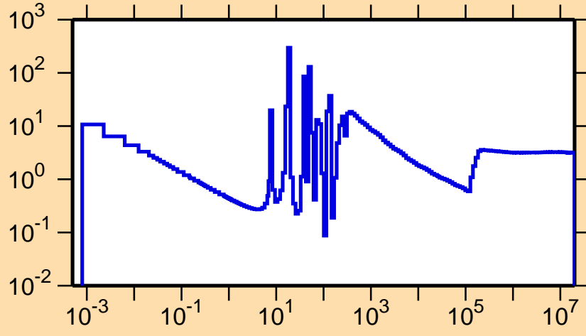
\sigma vs. E for ^{219}\text{At}(n,\text{nonel.})
