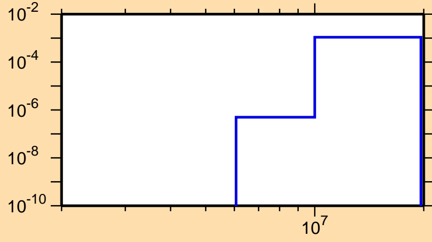
\sigma vs. E for ^{219}\text{At}(n,p)
