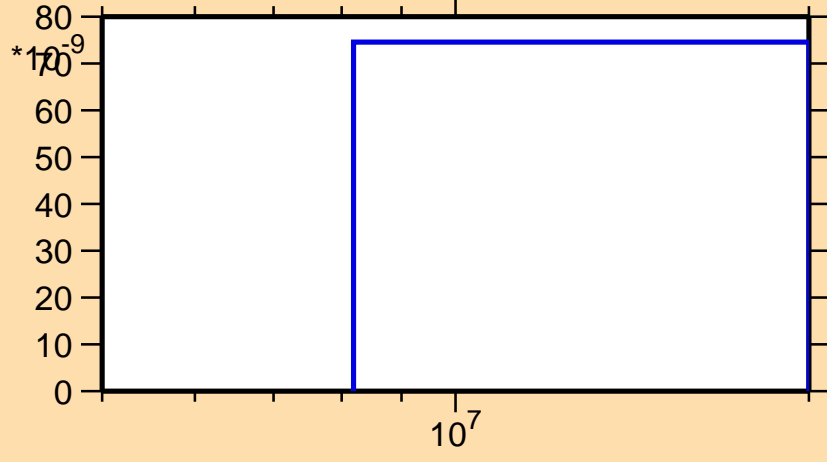
\sigma vs. E for ^{219}\text{At}(\text{mt117})
