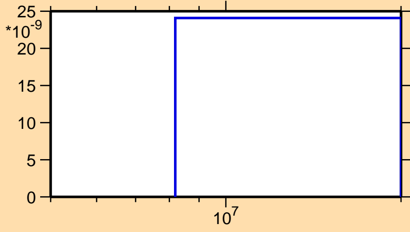
\sigma vs. E for ^{219}\text{At}(n,nt)
