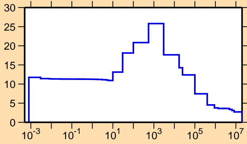
\sigma vs. E for ^{219}\text{At}(n,\text{el.})
