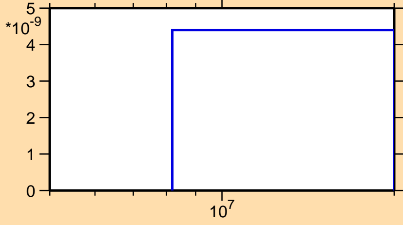
\sigma vs. E for ^{219}\text{At}(n,p\alpha)
