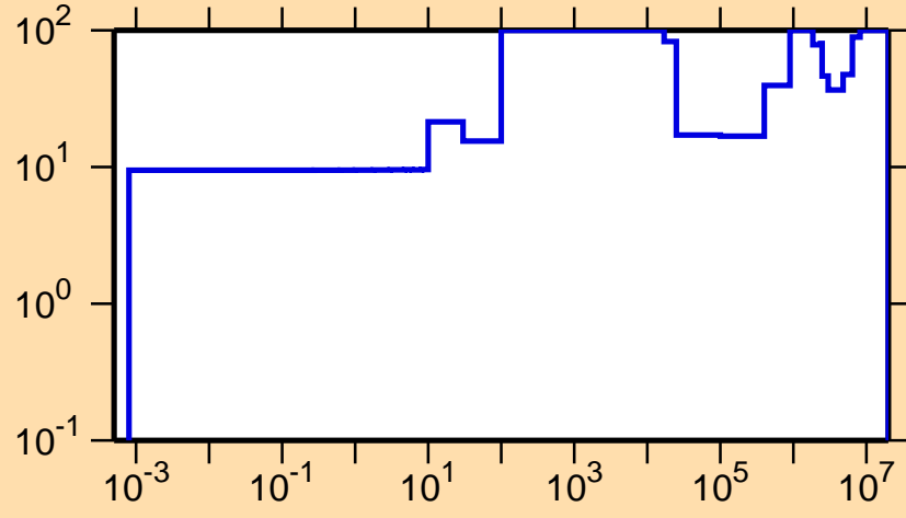
\Delta\sigma/\sigma vs. E for ^{219}\text{At}(n,el.)
