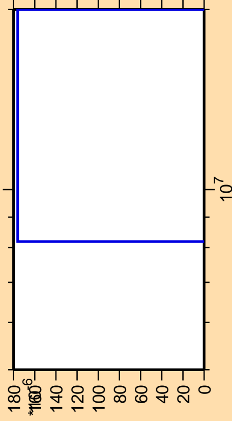
\Delta\sigma/\sigma vs. E for ^{219}\text{At}(\text{mt } 42)
