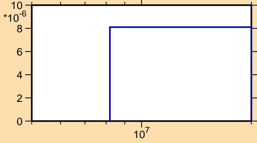
\sigma vs. E for ^{219}\text{At}(n,3n)
