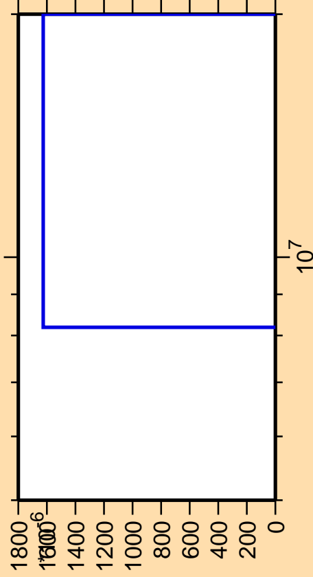
\Delta\sigma/\sigma vs. E for ^{219}\text{At}(\text{mt } 11)
