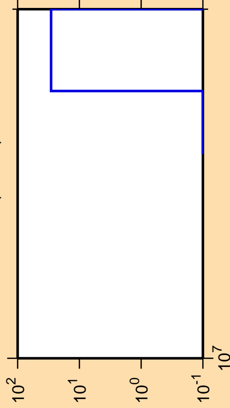
\Delta\sigma/\sigma vs. E for ^{220}\text{At} (mt 42)
