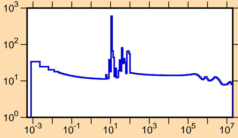
\sigma vs. E for ^{220}\text{At}(n,\text{tot.})
