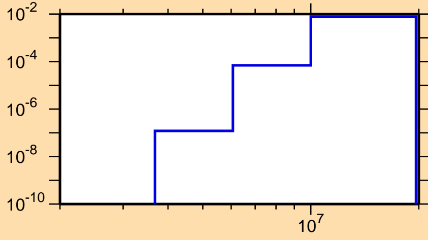
\sigma vs. E for ^{220}\text{At}(n,p)
