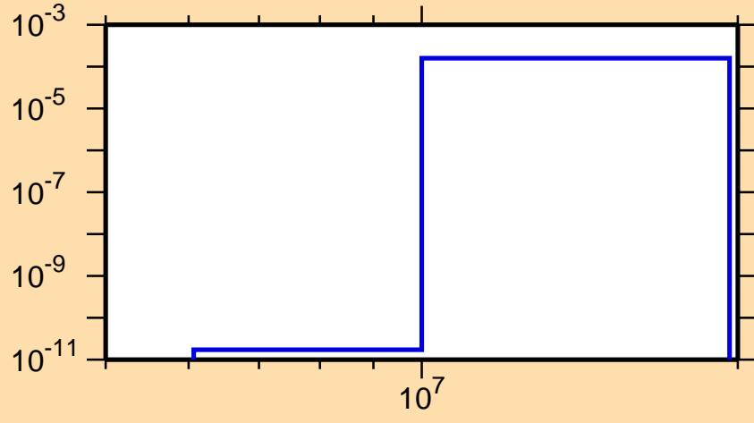
\sigma vs. E for ^{220}\text{At}(n,np)
