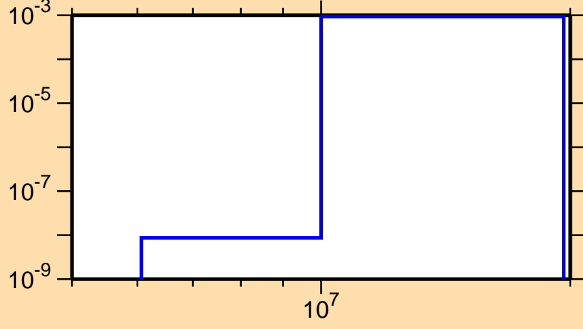
\sigma vs. E for ^{220}\text{At}(n,d)
