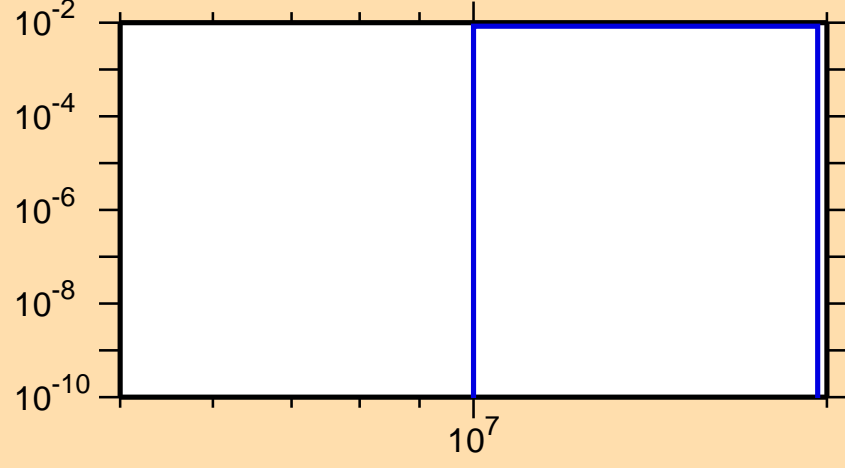
\sigma vs. E for ^{220}\text{At}(n,3n\alpha)
