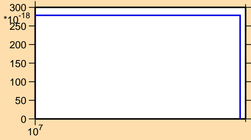
\sigma vs. E for ^{220}\text{At}(\text{mt } 34)
