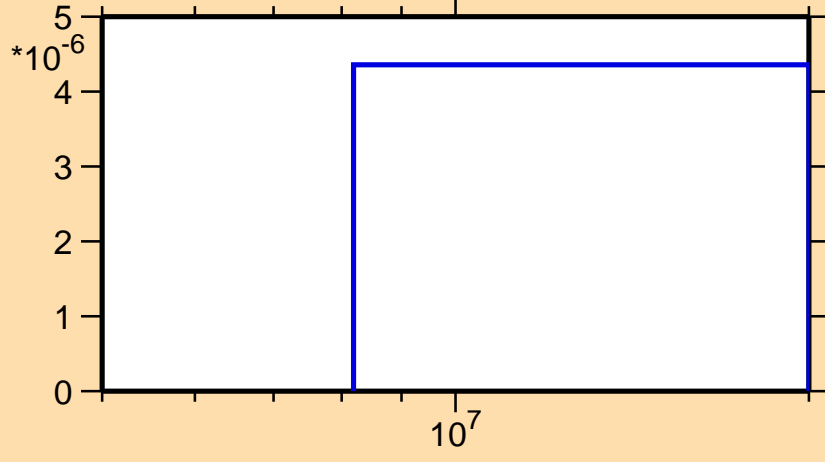
\sigma vs. E for ^{220}\text{At}(\text{mt117})
