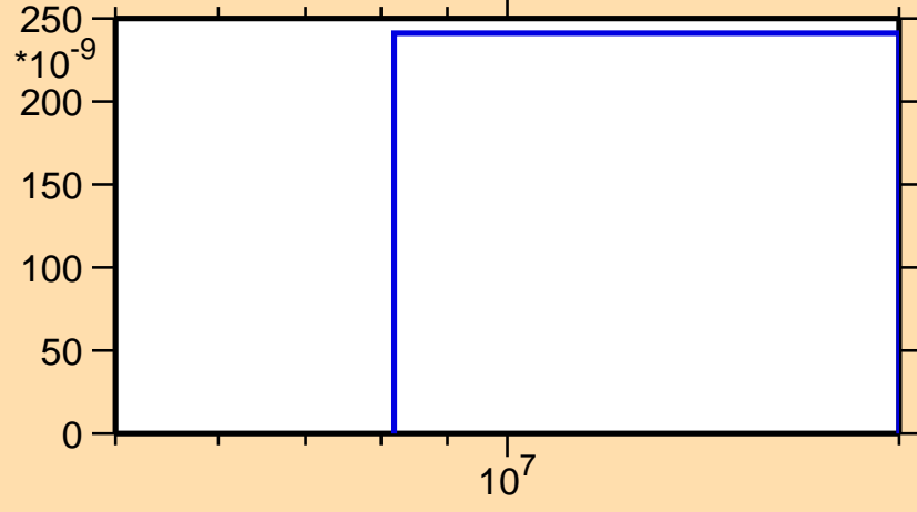
\sigma vs. E for ^{220}\text{At}(n,2np)
