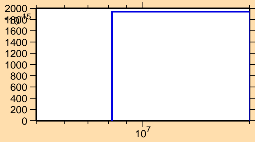
\sigma vs. E for ^{220}\text{At}(n,\text{He3})
