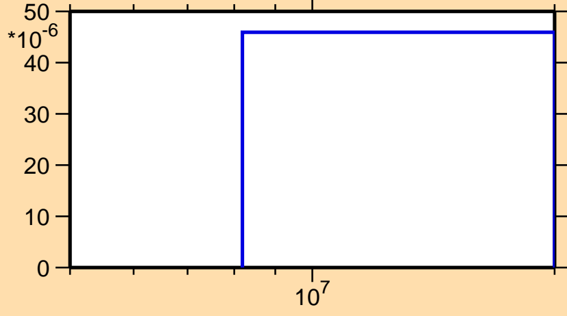
\sigma vs. E for ^{220}\text{At}(n,nt)
