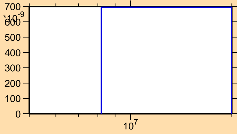
\sigma vs. E for ^{220}\text{At}(\text{mt } 45)
