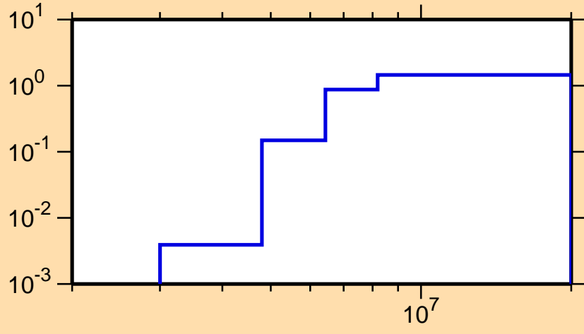
\sigma vs. E for ^{220}\text{At}(n,2n)
