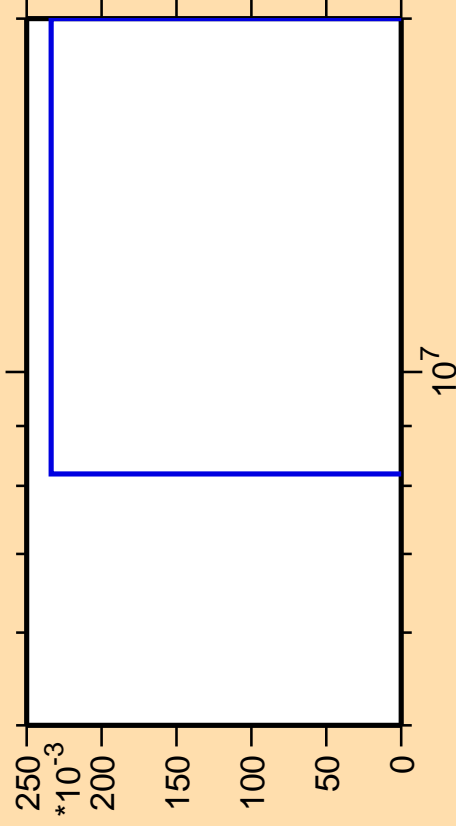
\Delta\sigma/\sigma vs. E for ^{220}\text{At}(\text{mt } 42)
