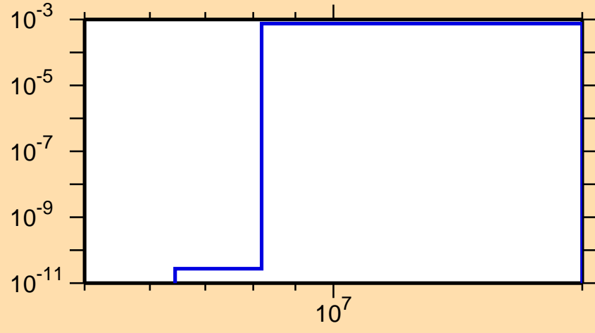
\sigma vs. E for ^{220}\text{At}(n,d)
