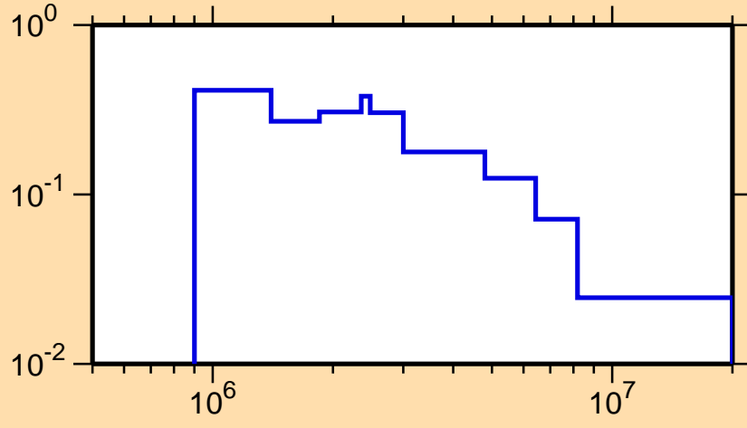
\sigma vs. E for ^{220}\text{At}(n,n\alpha)
