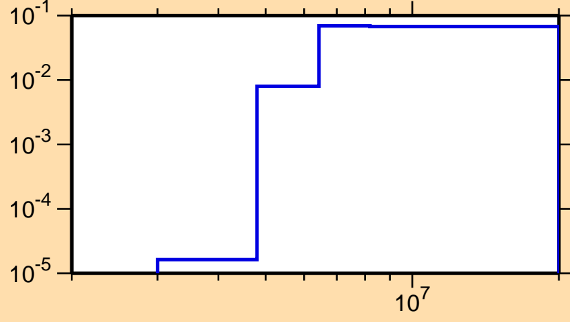
\sigma vs. E for ^{220}\text{At}(n,2n\alpha)
