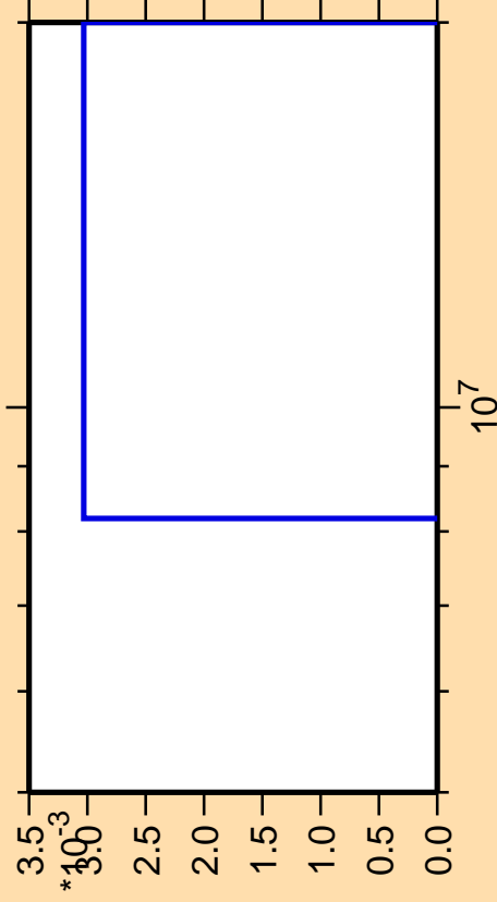
\Delta\sigma/\sigma vs. E for ^{220}\text{At}(\text{mt } 34)
