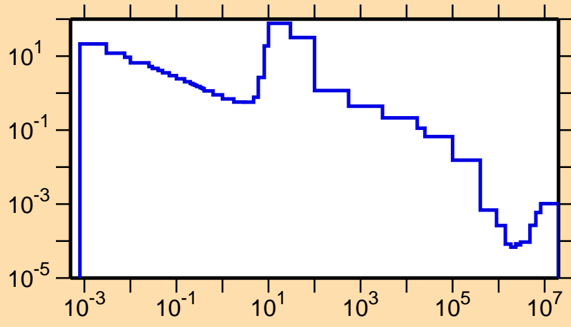
\sigma vs. E for ^{220}\text{At}(n,\gamma)
