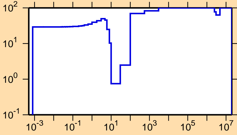
\Delta\sigma/\sigma vs. E for ^{220}\text{At}(n,\gamma)
