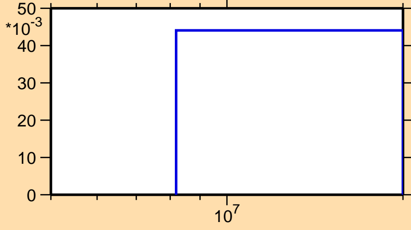
\sigma vs. E for ^{220}\text{At}(n,3n)
