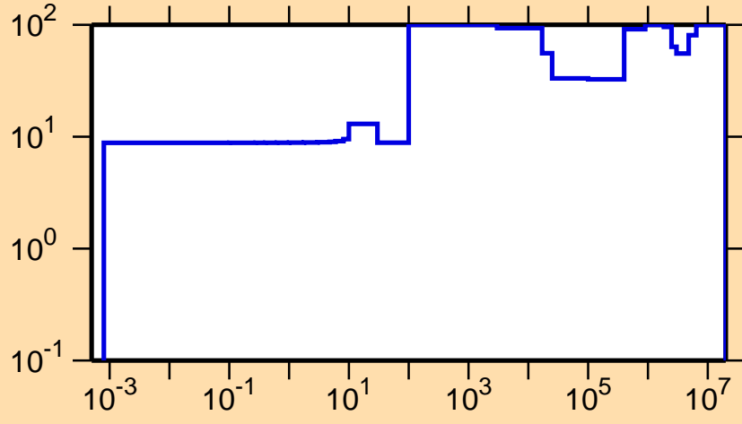
\Delta\sigma/\sigma vs. E for ^{220}\text{At}(n,el.)
