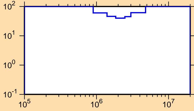
\Delta\sigma/\sigma vs. E for ^{220}\text{At}(n,n\text{cont.})
