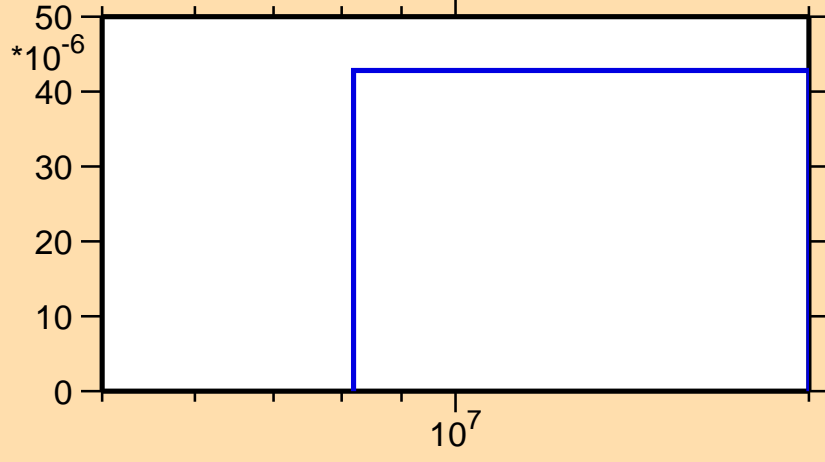
\sigma vs. E for ^{220}\text{At}(n,p\alpha)
