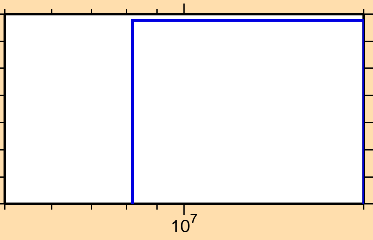
\sigma vs. E for ^{220}\text{At}(n,3n\alpha)
