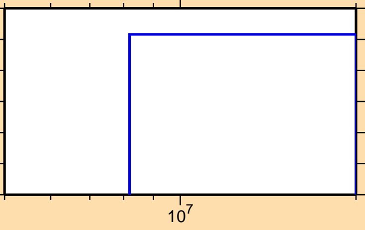
\sigma vs. E for ^{220}\text{At}(n,\text{nd})
