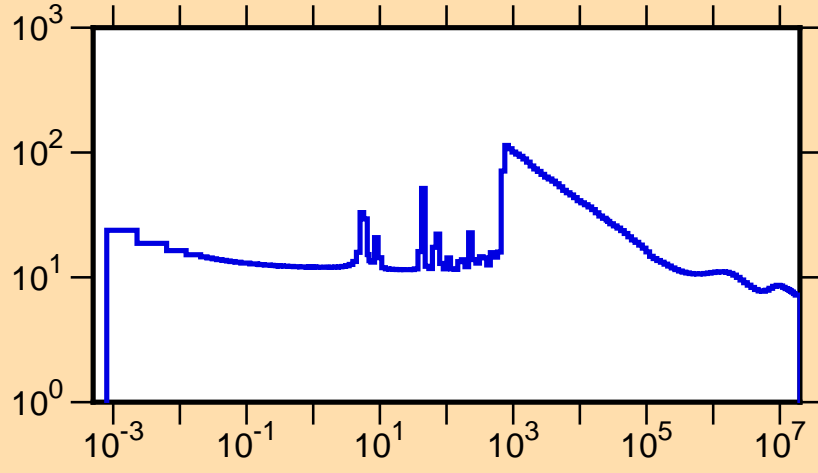
\sigma vs. E for ^{221}\text{At}(n,\text{tot.})
