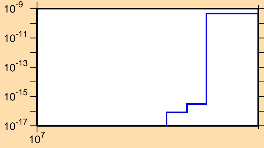
\sigma vs. E for ^{221}\text{At}(\text{mt } 42)
