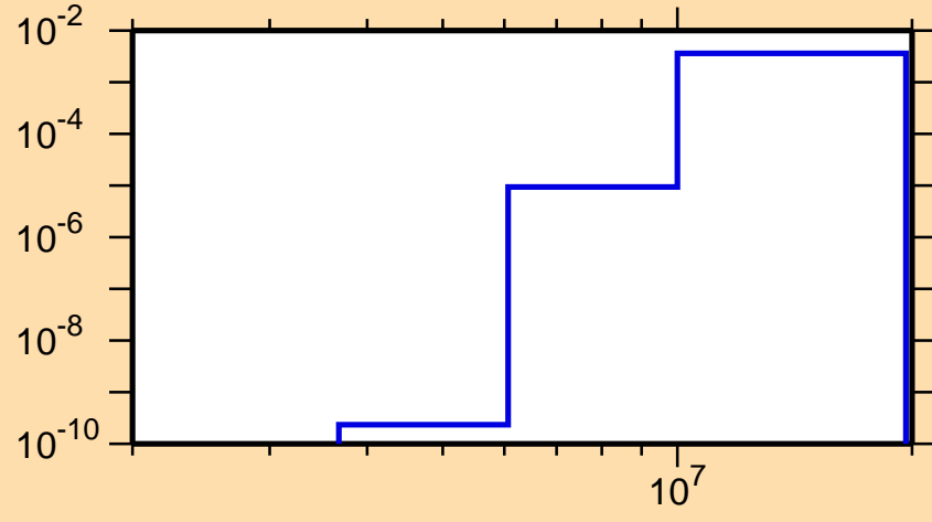
\sigma vs. E for ^{221}\text{At}(n,p)
