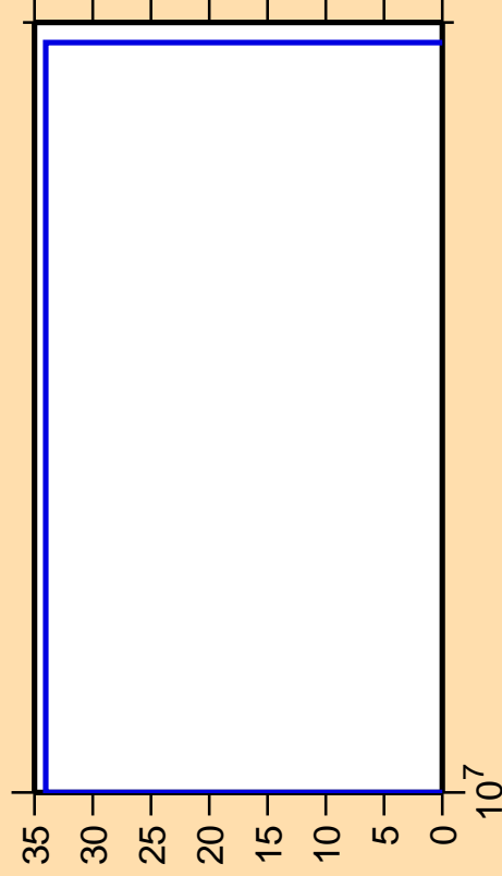
\Delta\sigma/\sigma vs. E for ^{221}\text{At} (mt 45)
