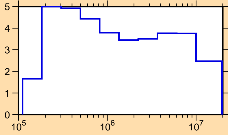
\sigma vs. E for ^{221}\text{At}(n,\text{inel.})
