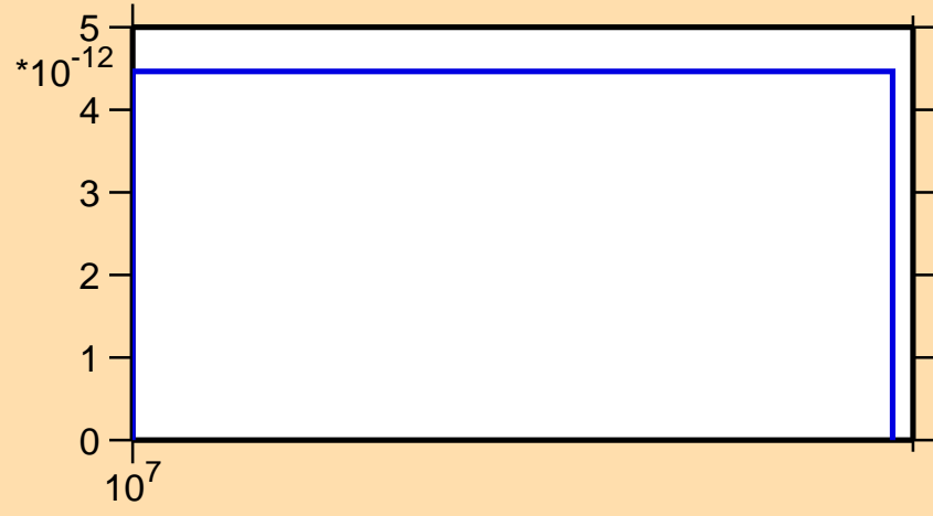
\sigma vs. E for ^{221}\text{At} (mt 45)
