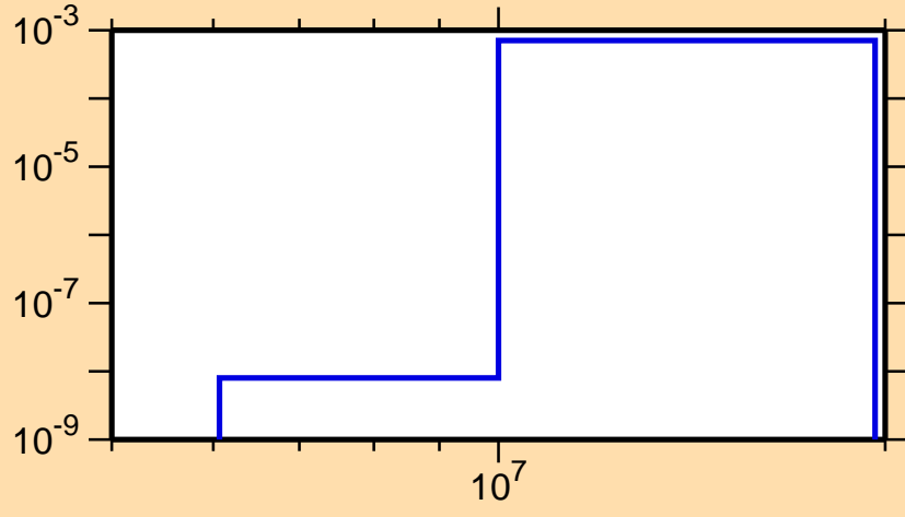
\sigma vs. E for ^{221}\text{At}(n,t)
