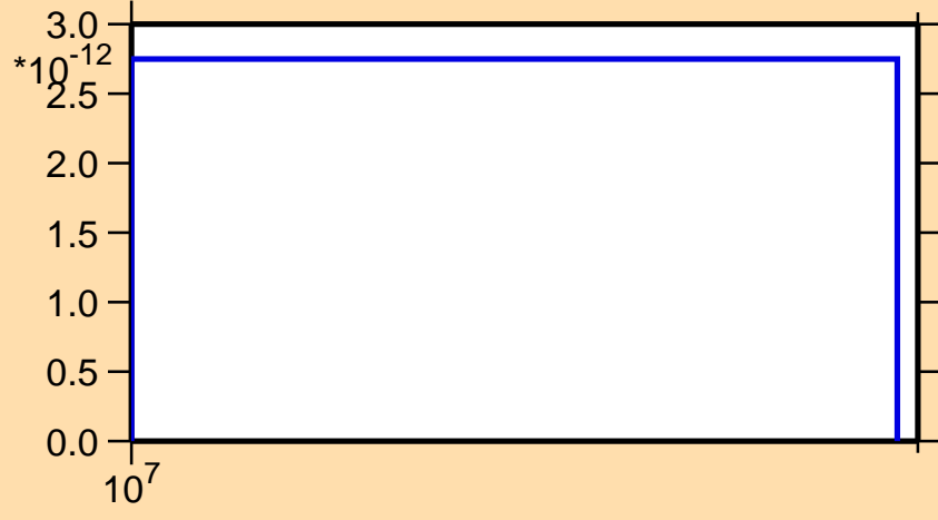
\sigma vs. E for ^{221}\text{At} (mt 42)
