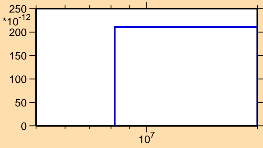
\sigma vs. E for ^{221}\text{At}(\text{mt } 11)
