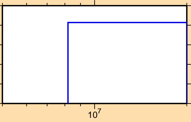
\sigma vs. E for ^{221}\text{At}(\text{mt } 45)
