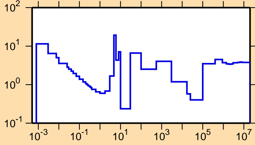
\sigma vs. E for ^{221}\text{At}(n,\text{nonel.})
