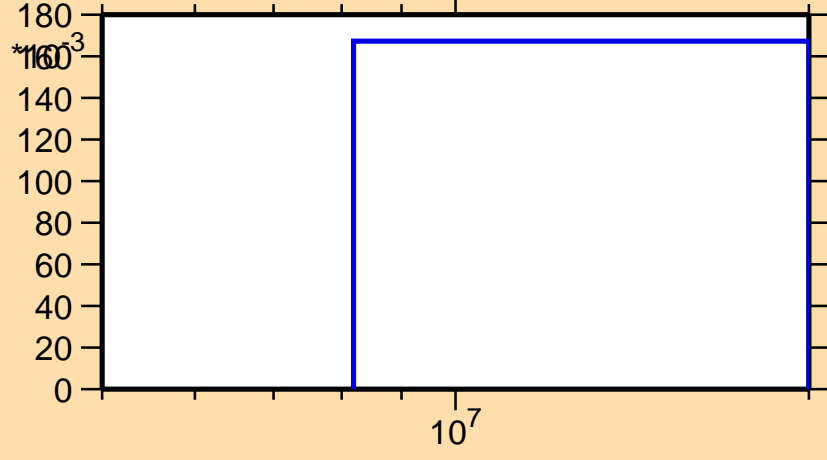
\sigma vs. E for ^{221}\text{At}(n,3n)
