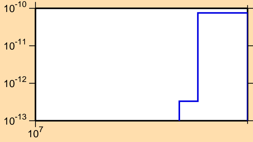
\sigma vs. E for ^{222}\text{At}(n,\text{He3})
