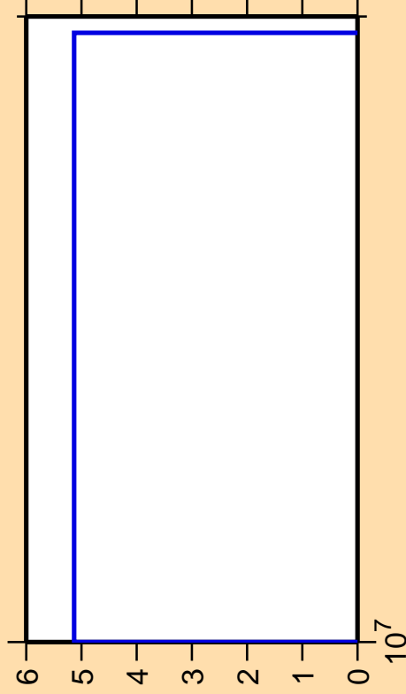
\Delta\sigma/\sigma vs. E for ^{222}\text{At}(n,\text{He3})
