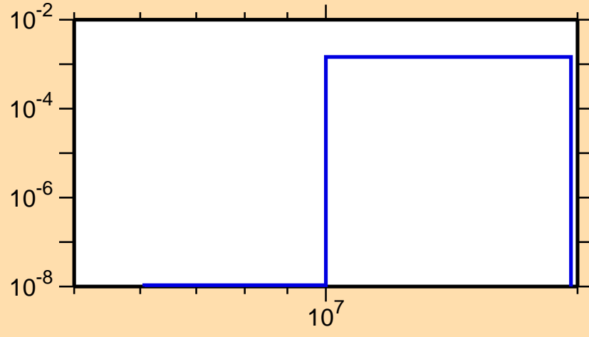
\sigma vs. E for ^{222}\text{At}(n,d)
