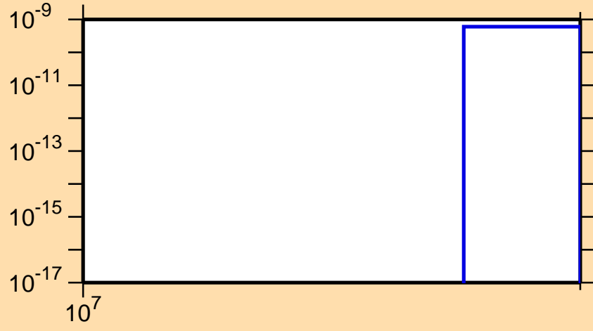
\sigma vs. E for ^{223}\text{At} (mt 42)
